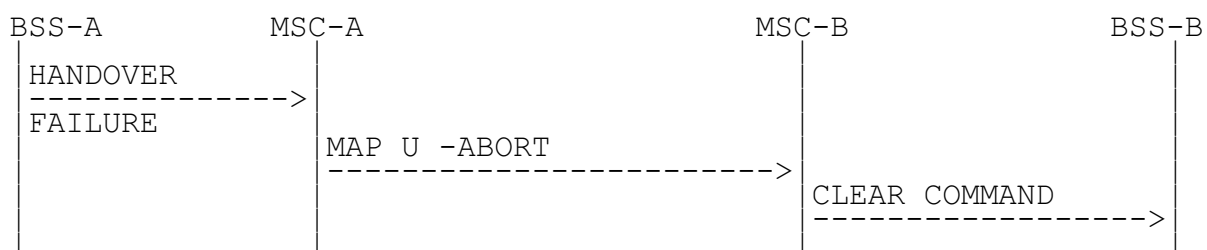
Figure 7: Signalling for Basic Inter-MSC Handover execution (Negative outcomes)
