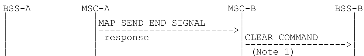
Figure 9: Signalling for Basic Inter-MSC Handover completion (Positive outcome)
