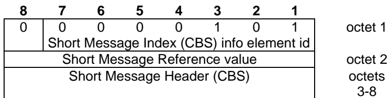
Figure 2.5.7/GSM 07.05: Short Message Index (CBS) information element
