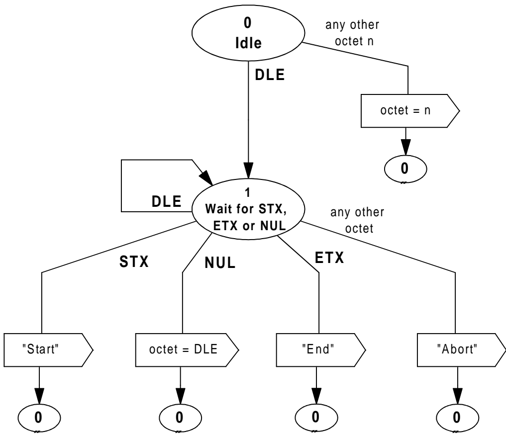
State transitions in Stage 1
