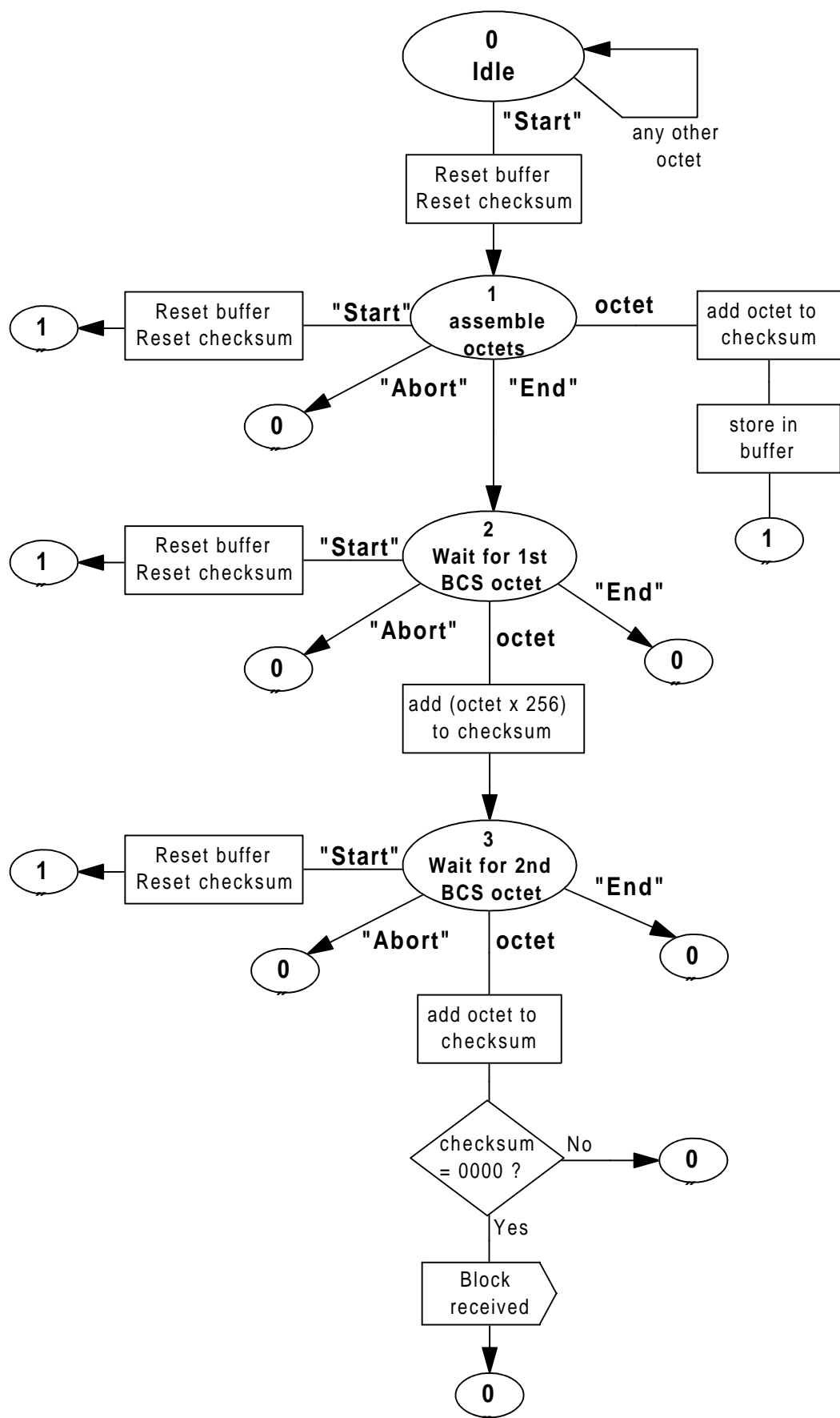
State transitions in Stage 2
