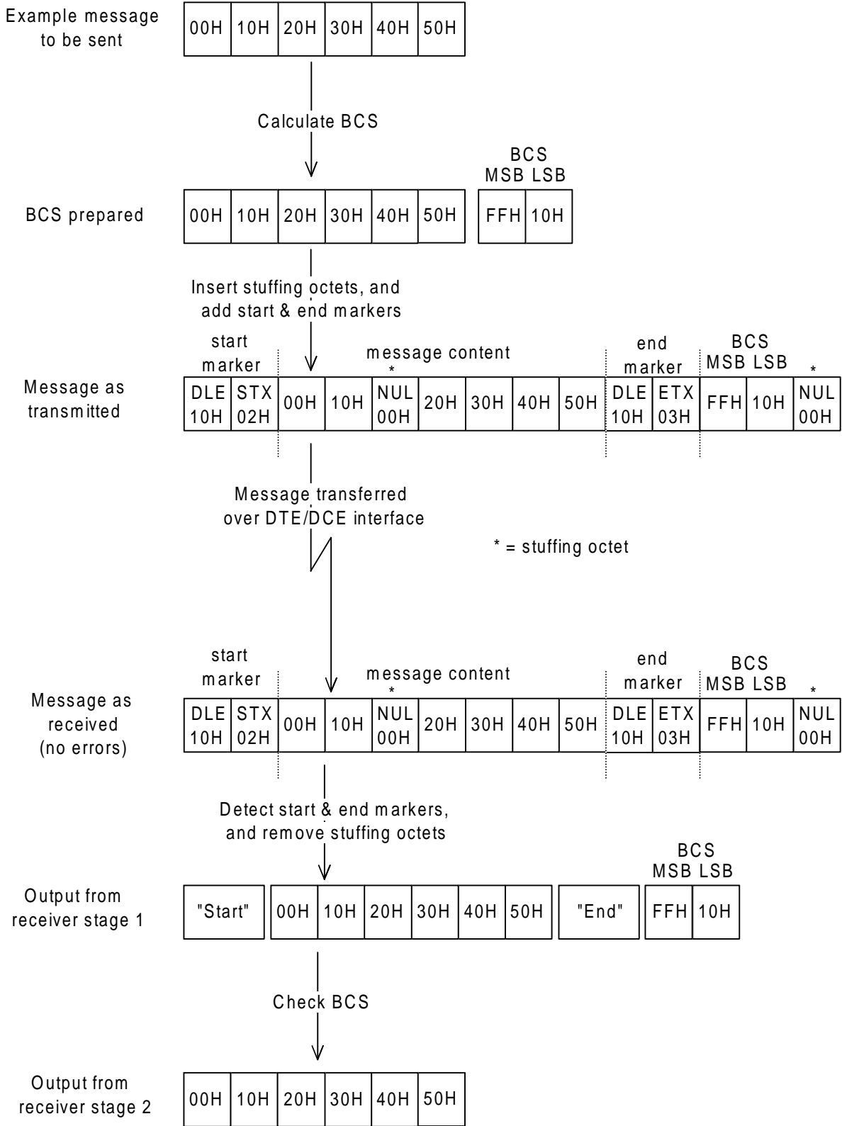
Example of coding / decoding a message at the DTE/DCE interface
