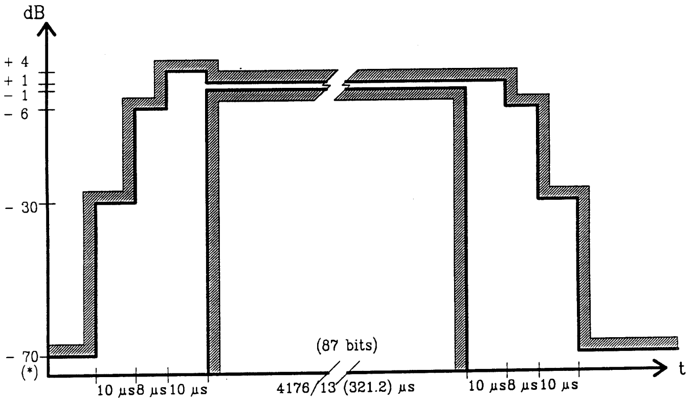
Time mask for access burst (AB)
