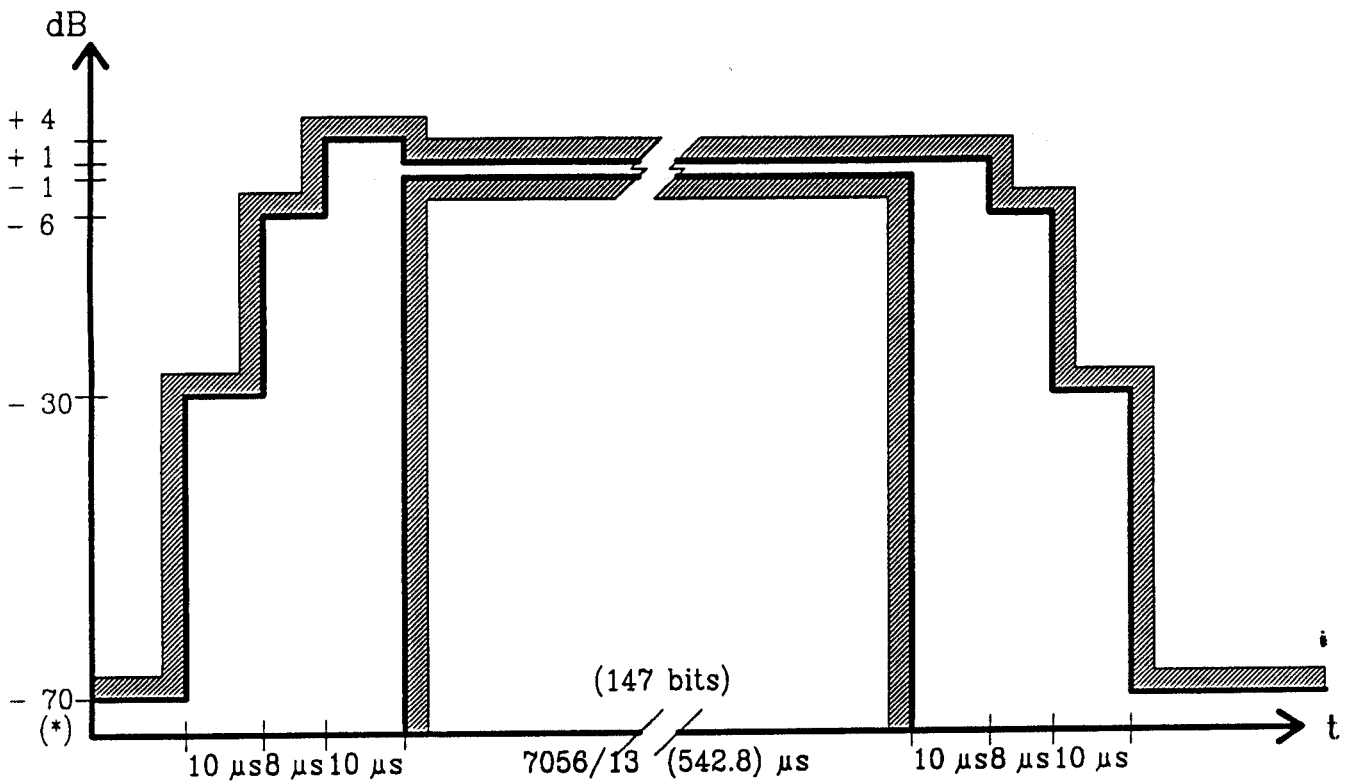
Time mask for normal duration bursts (NB, FB, DB and SB)
