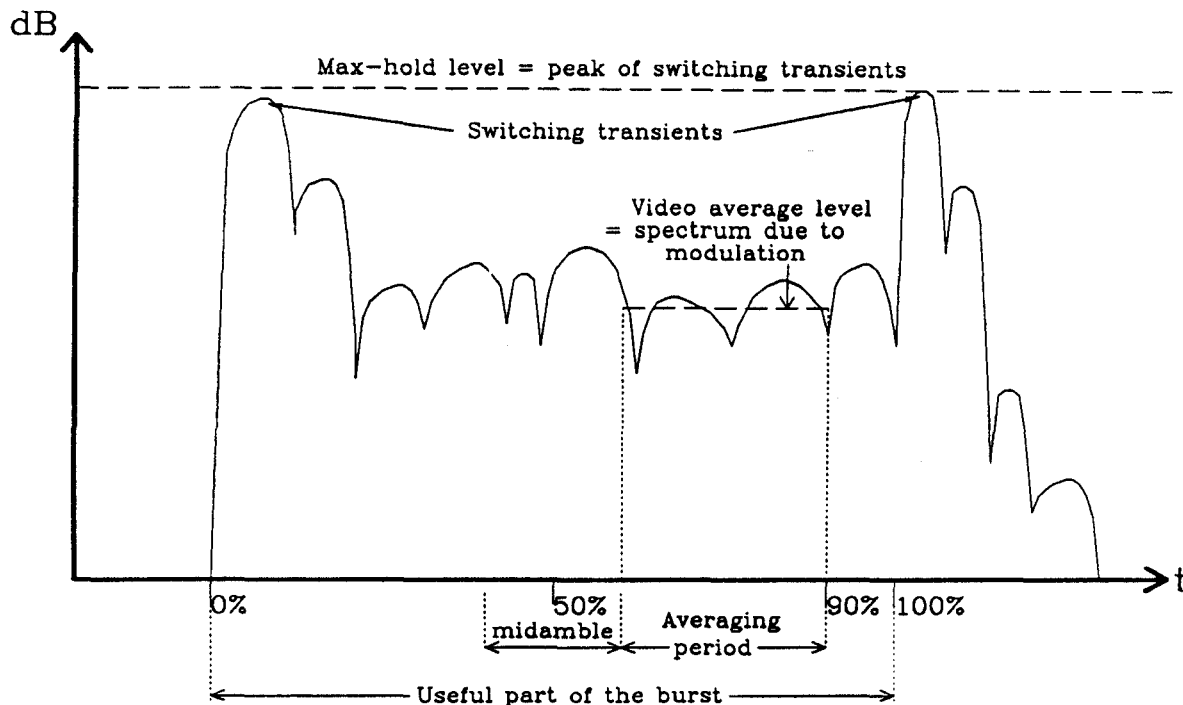
Figure 1: Example of a time waveform due to a burst as seen in a 30 kHz filter offset from the carrier.
