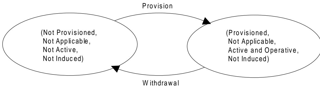
Figure 10: State transition model
