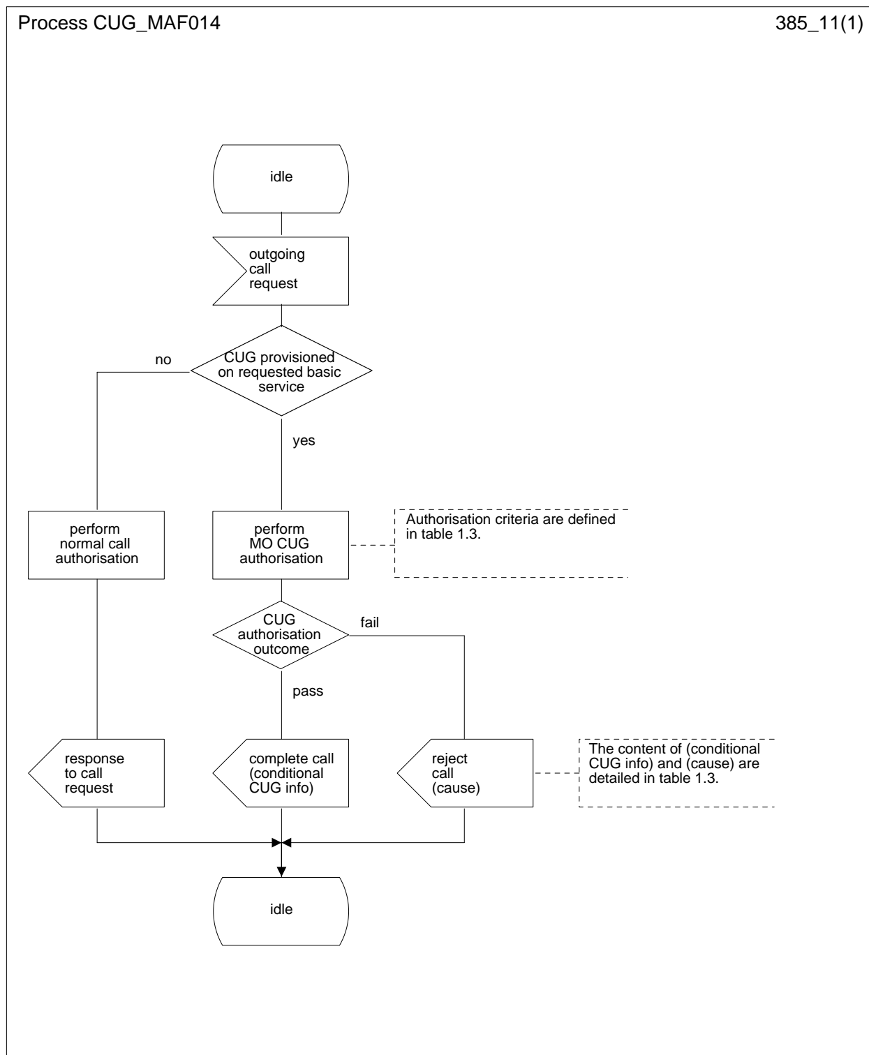
Figure 1.1: MAF014 Mobile Originated CUG call authorization (VLR)
