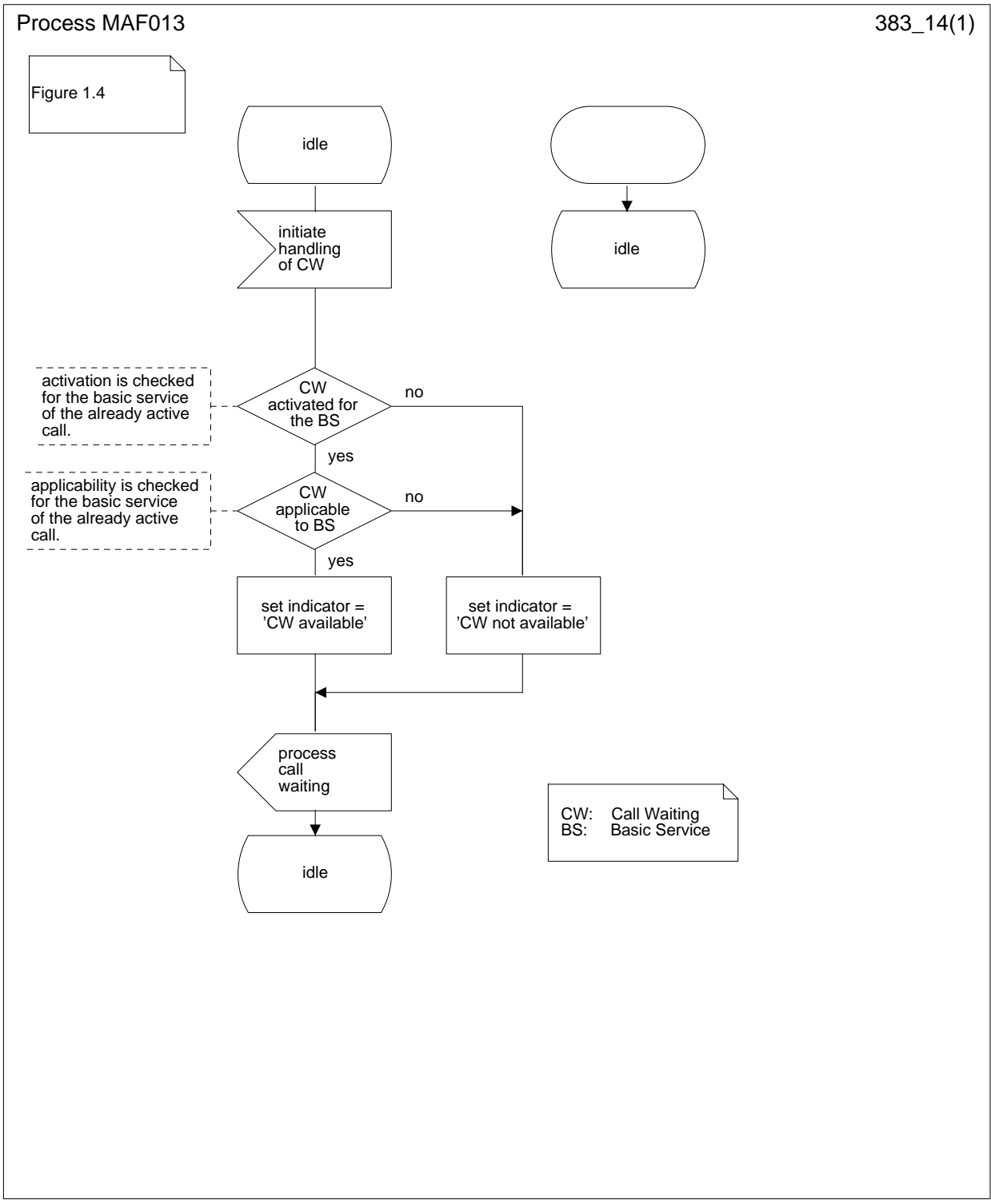
Figure 1.4: MAF013 Call waiting related authorizations examination (VLR)
