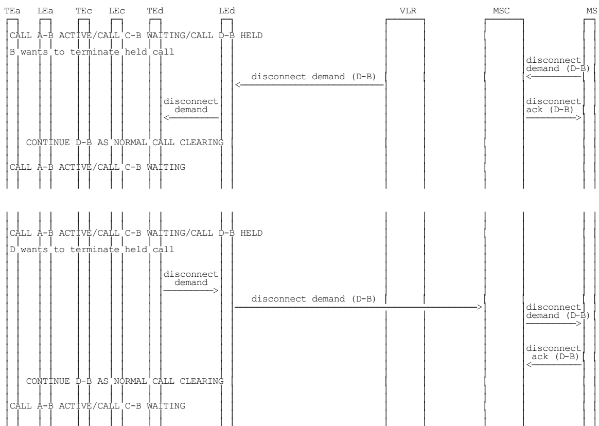
Figure 1.6 (sheet 7 of 7): Information flow for call waiting
