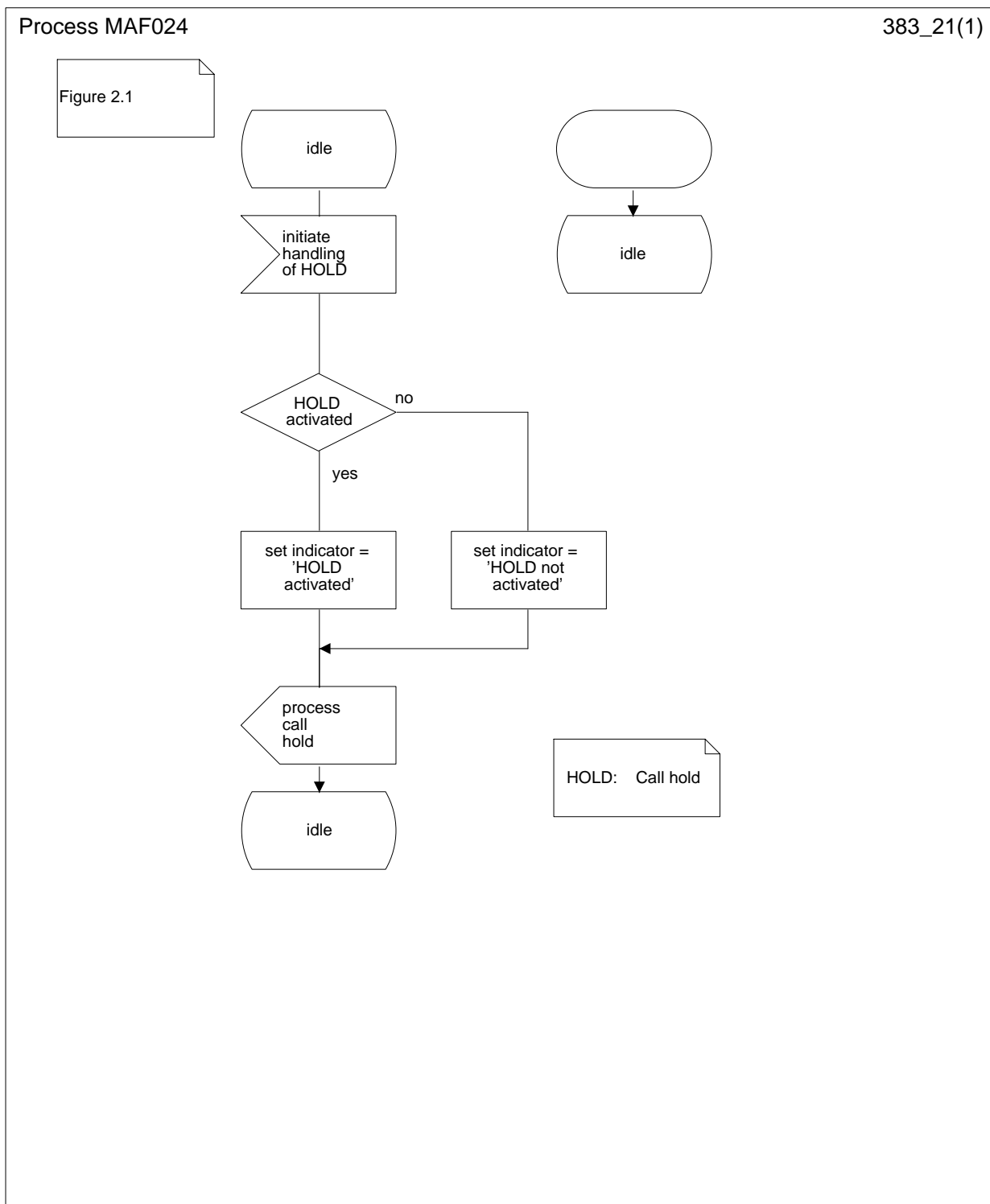
Figure 2.1: MAF024 Call hold related authorizations examination (VLR)
