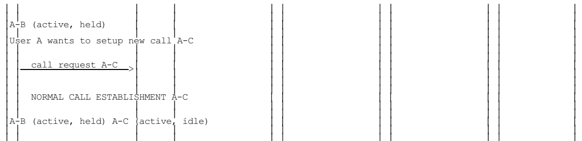
Figure 2.3 (sheet 1 of 3): Information flow for call hold
