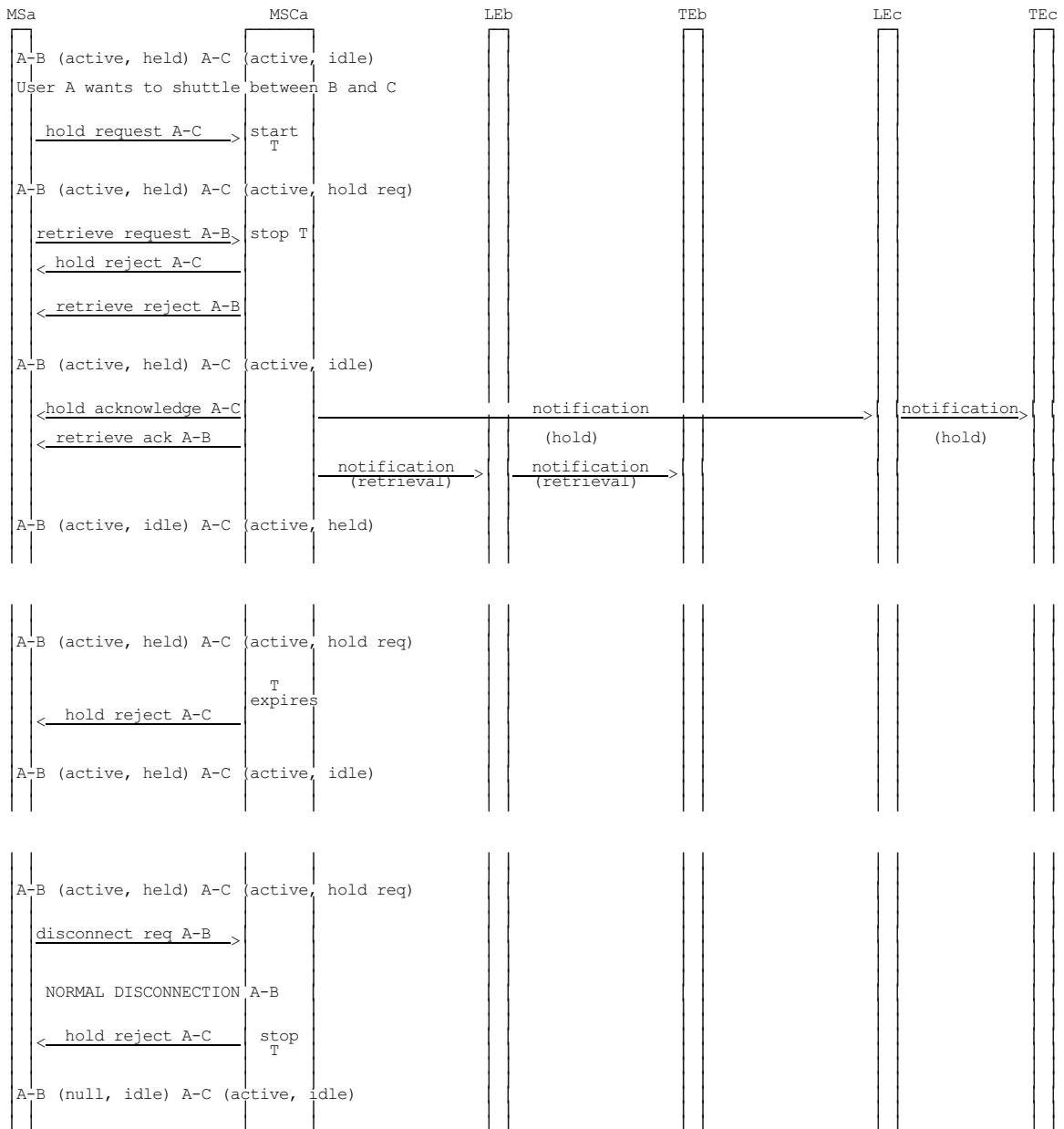
Figure 2.3 (sheet 2 of 3): Information flow for call hold
