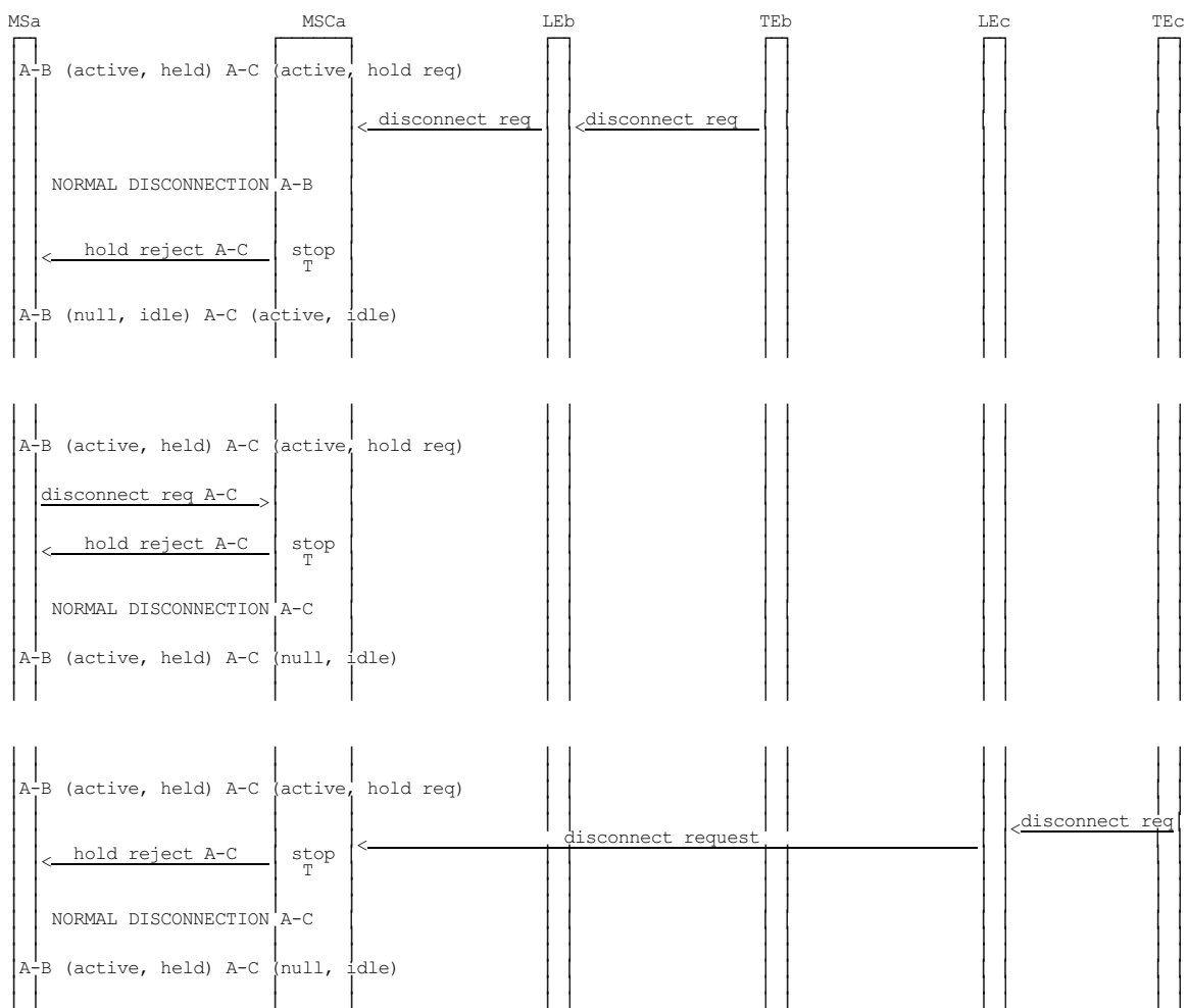
Figure 2.3 (sheet 3 of 3): Information flow for call hold
