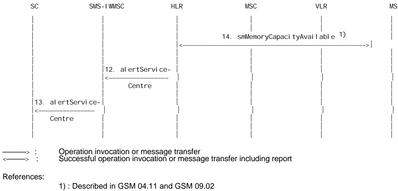
Figure 03.40/20c; The alert procedure when the MS notifies the network that it has memory available to receive one or more short messages and MCEF is set.
