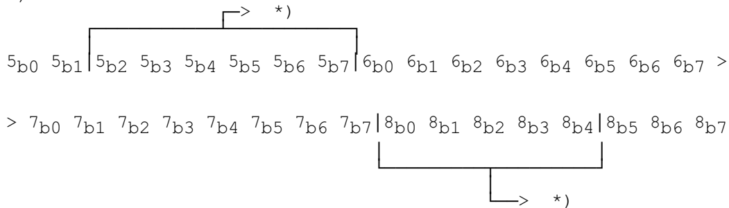
Figure 03.40/8: 21 bits from the octets 5, 6, 7, and 8 in a short message α) will represent an integer as shown in β), and will be transmitted in an order as shown in Γ).
