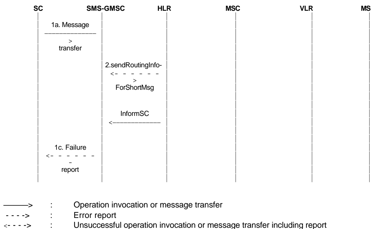
Figure 03.40/15c): Short message transfer attempt failing due to negative outcome of HLR information retrieval.
