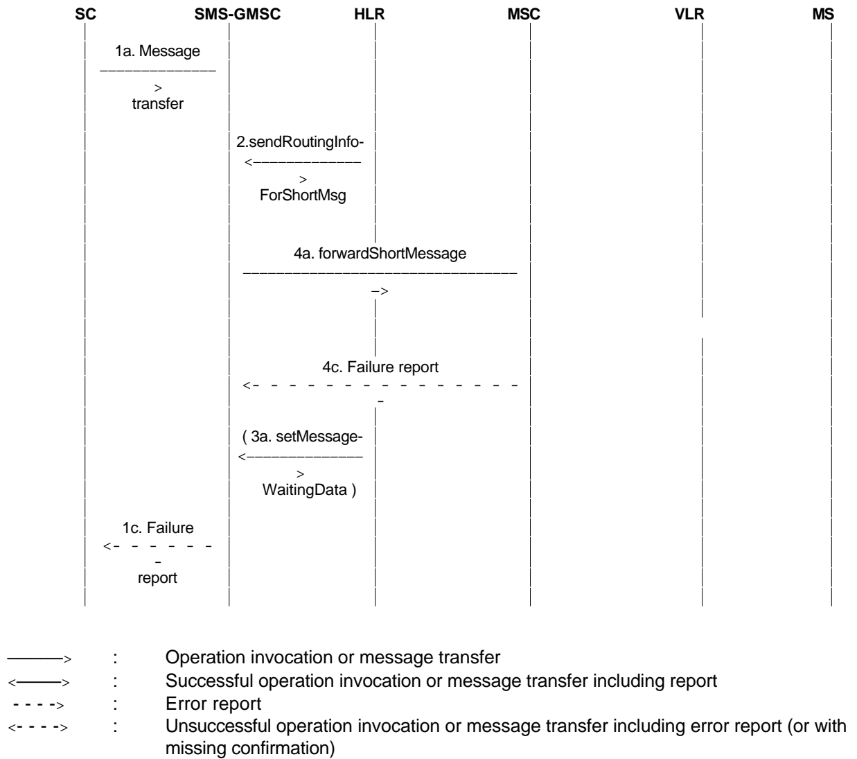
Figure 03.40/15d): Short message transfer attempt failing due to error at the MSC.
