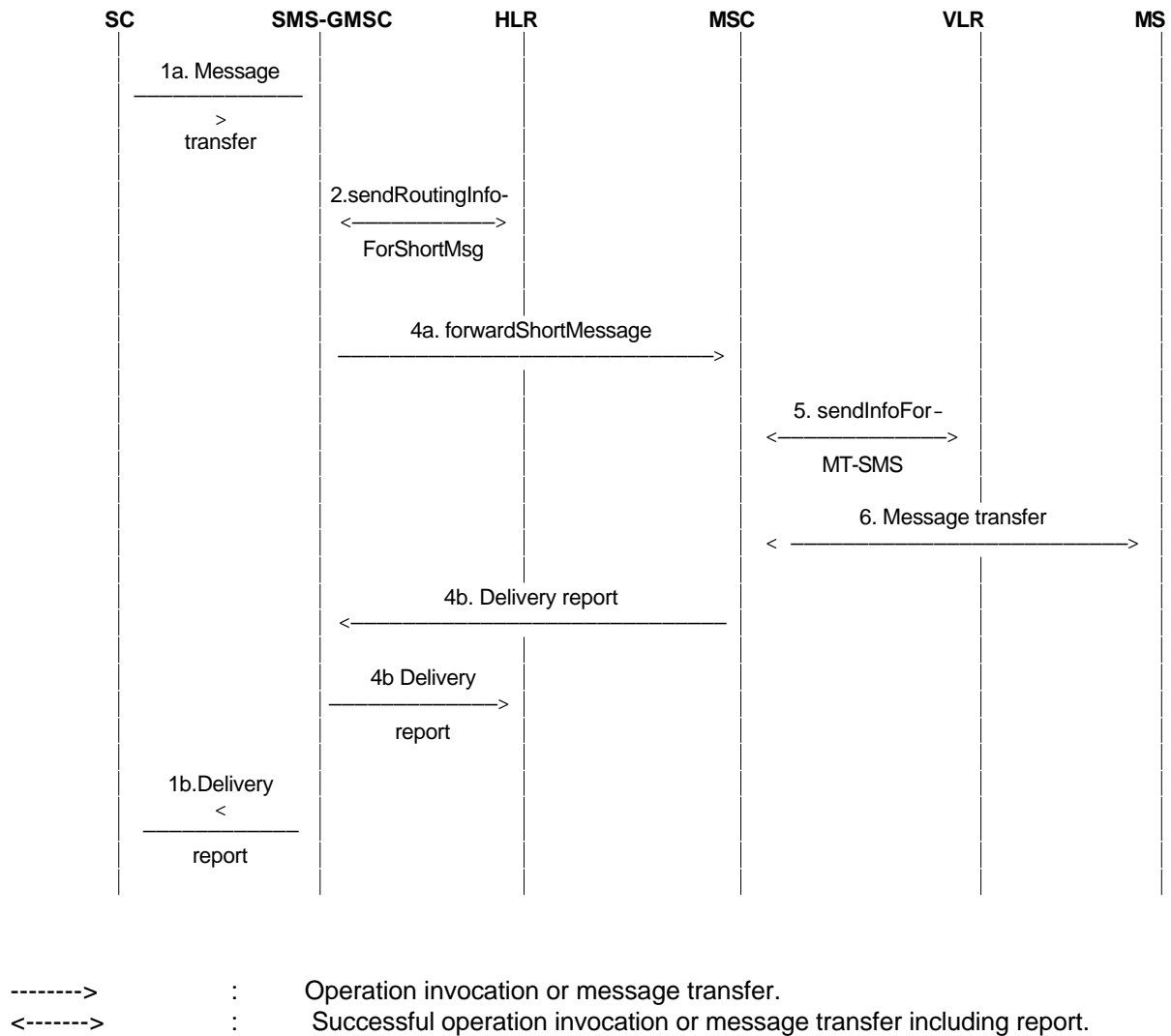
Figure 03.40/15a): Successful short message transfer attempt.
