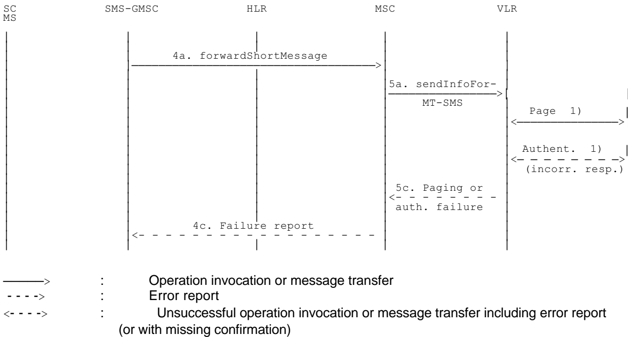
Figure 03.40/16c): 'Send information for MT SMS' procedure; erroneous case: Absent subscriber (e.g. no paging response).
