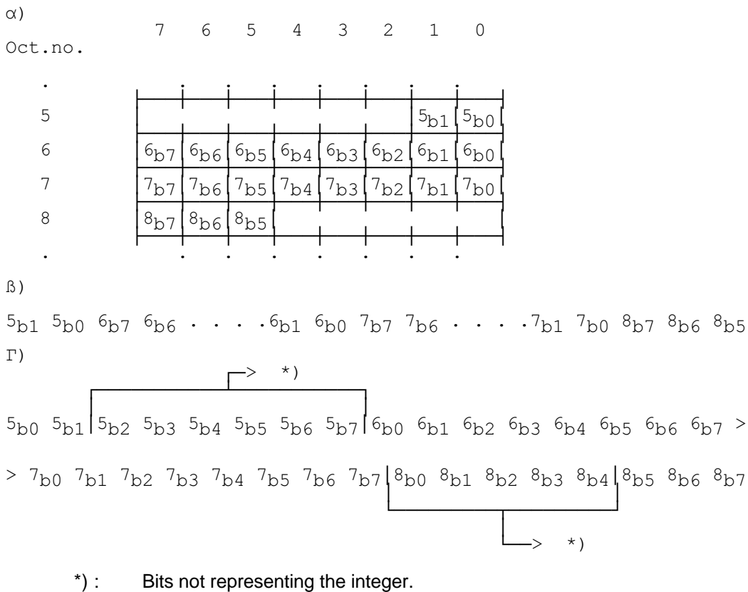
Figure 03.40/8: 21 bits from the octets 5, 6, 7, and 8 in a short message α) will represent an integer as shown in β), and will be transmitted in an order as shown in Γ).
