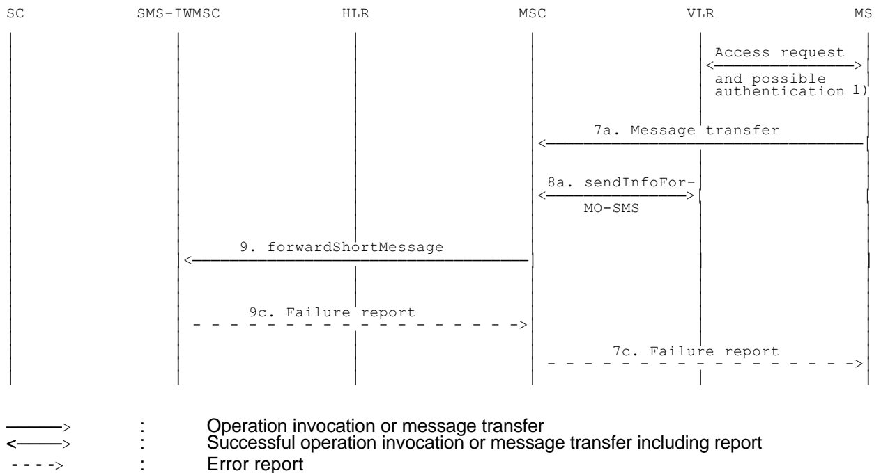
Figure 03.40/18c): Short message transfer attempt failing due to negative outcome of VLR information retrieval.
