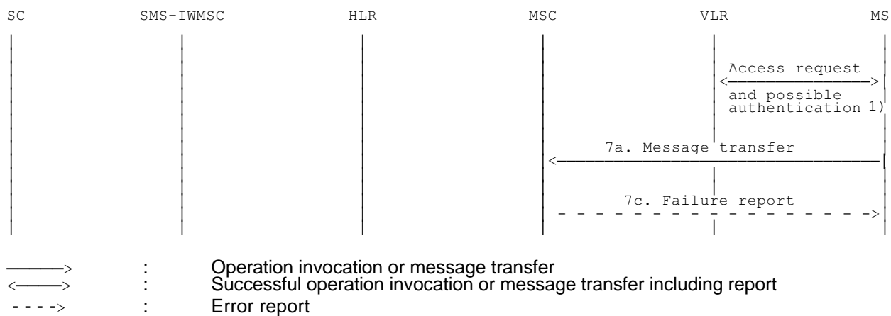
Figure 03.40/18a): Successful short message transfer attempt.
