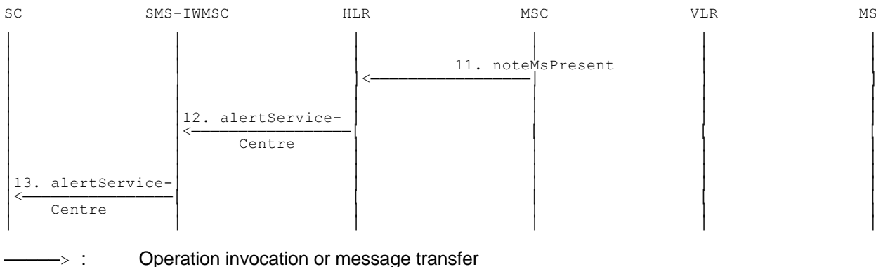
Figure 03.40/20a: The alert procedure when the MS becomes reachable, MNRF is set and MCEF is not set.
