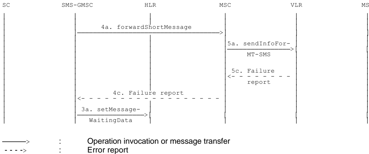
Figure 03.40/16b): 'Send information for MT SMS' procedure; erroneous case: absent subscriber (e.g. IMSI DETACH).
