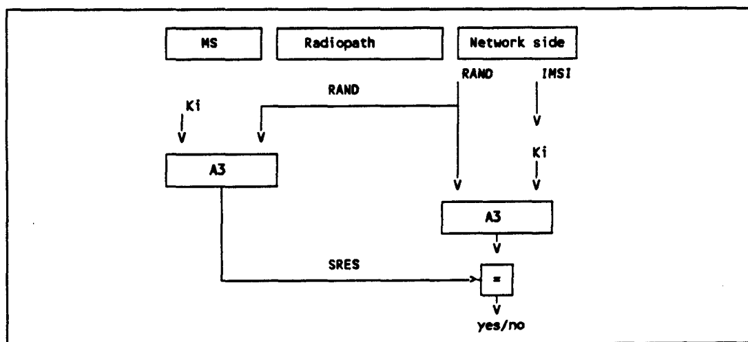
Figure 3.1 / GSM 03.20
