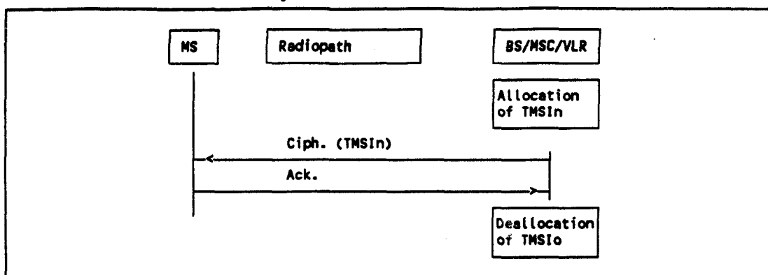
Figure 2.4 /GSM 03.20
