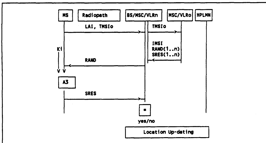
Figure 3.4 / GSM 03.20
