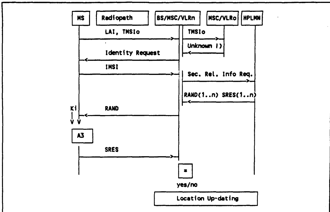
Figure 3.6 / GSM 03.20
