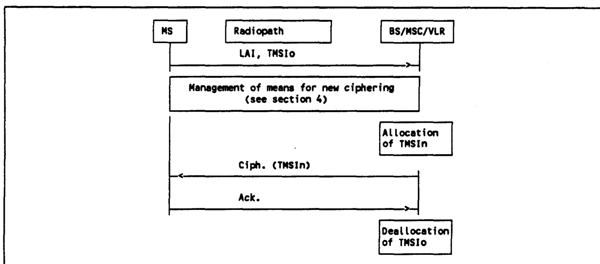
Figure 2.1 / GSM 03.20
