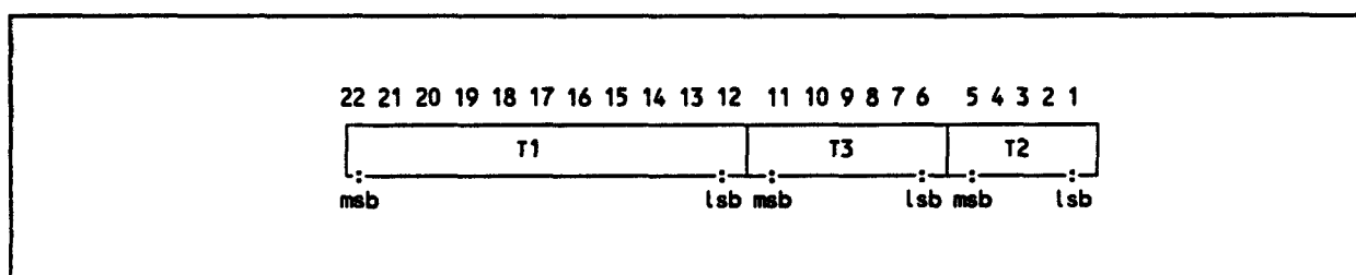
Figure 1.1a/GSM 03.20-Annex 3
