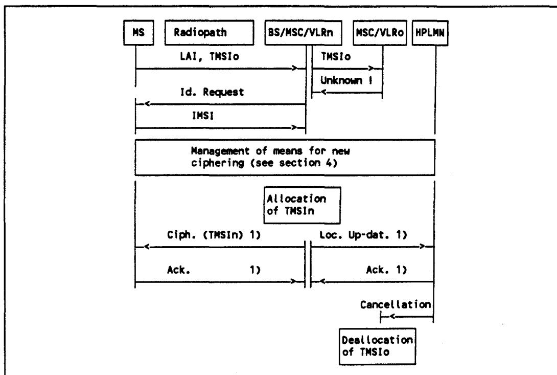
Figure 2.6 / GSM 03.20
