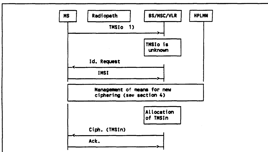
Figure 2.5 /GSM 03.20
