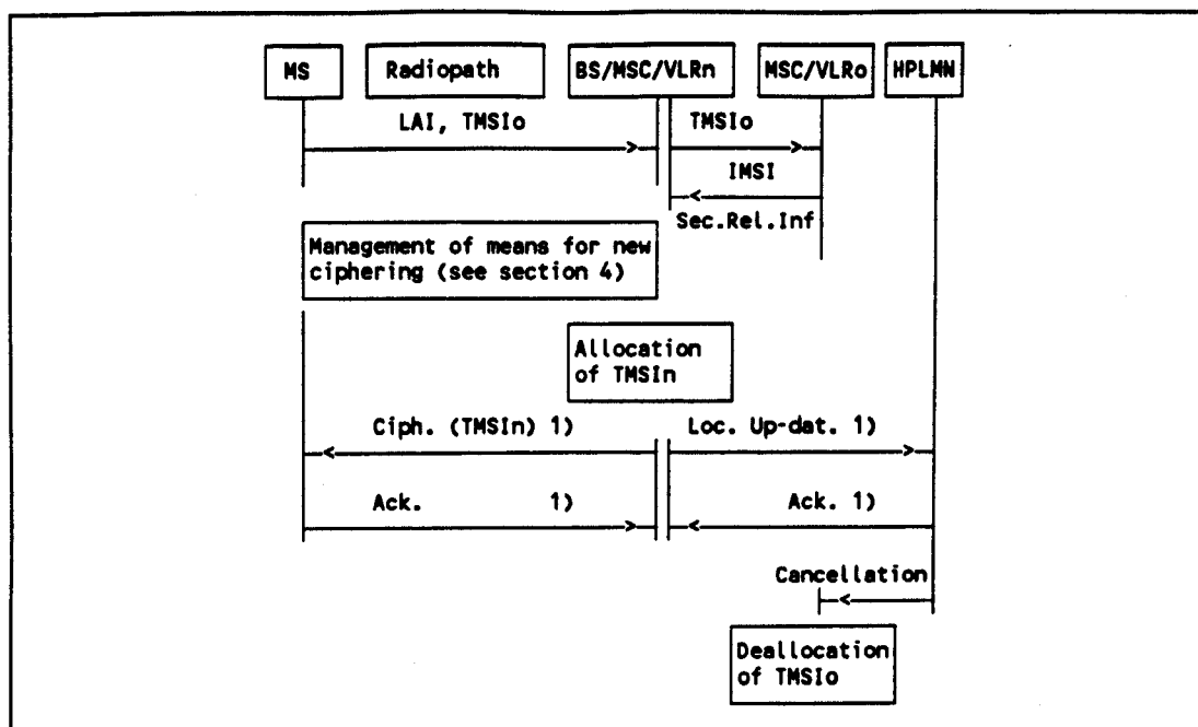
Figure 2.3 /GSM 03.20
