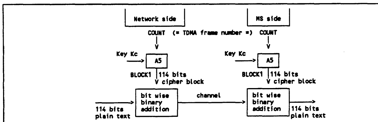
Figure 1.1 / GSM 03.20 - Annex 3 Decipherment on the MS side.
