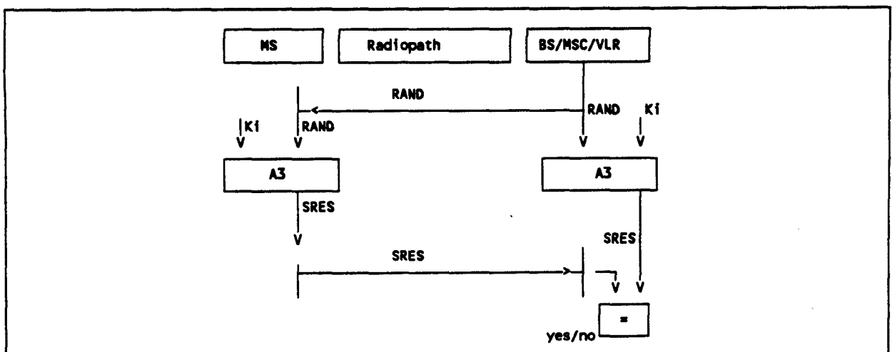
Figure 3.7 / GSM 03.20
