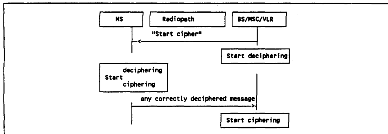
Figure 4.2 / GSM 03.20
