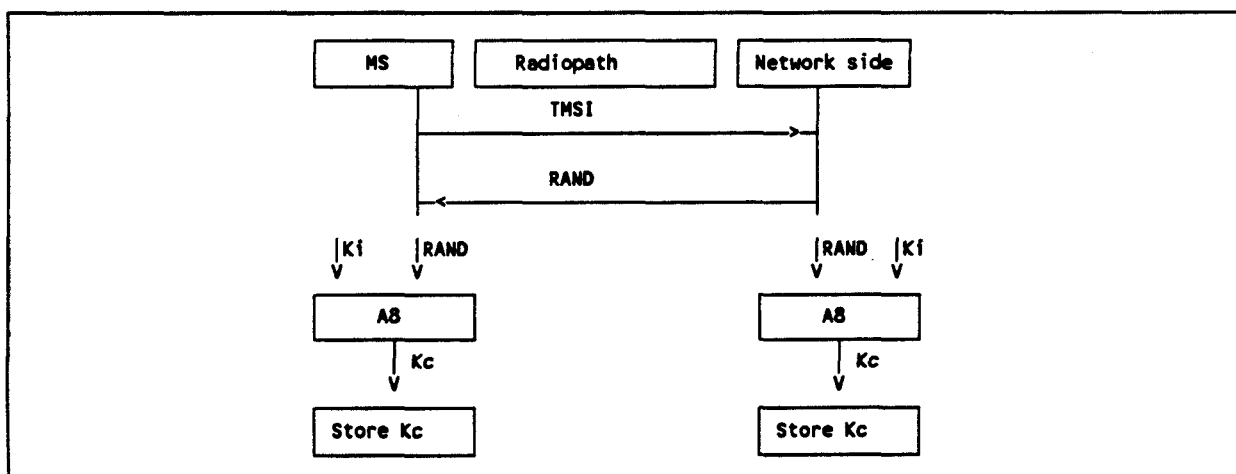
Figure 4.1 / GSM 03.20
