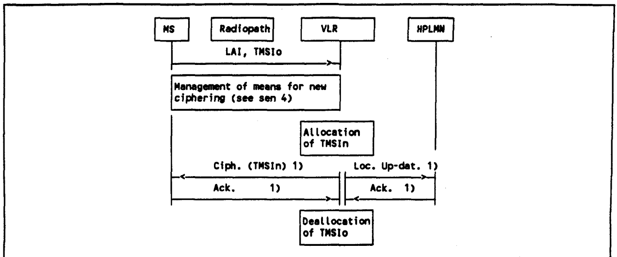
Figure 2.2 / GSM 03.20
