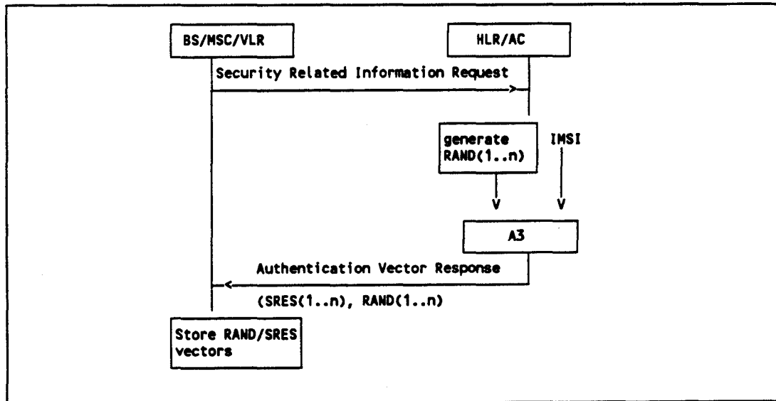
Figure 3.2 / GSM 03.20
