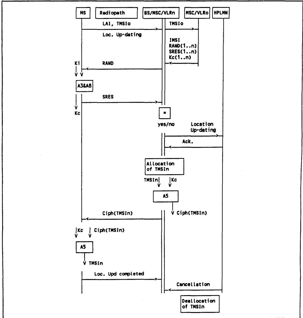
Figure 5.1 / GSM 03.20
