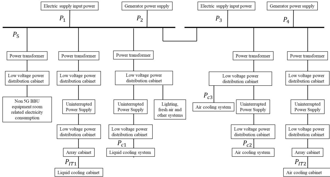
Figure 8: Configuration of calculation of the Cooling Effectiveness ( CoolEff )
