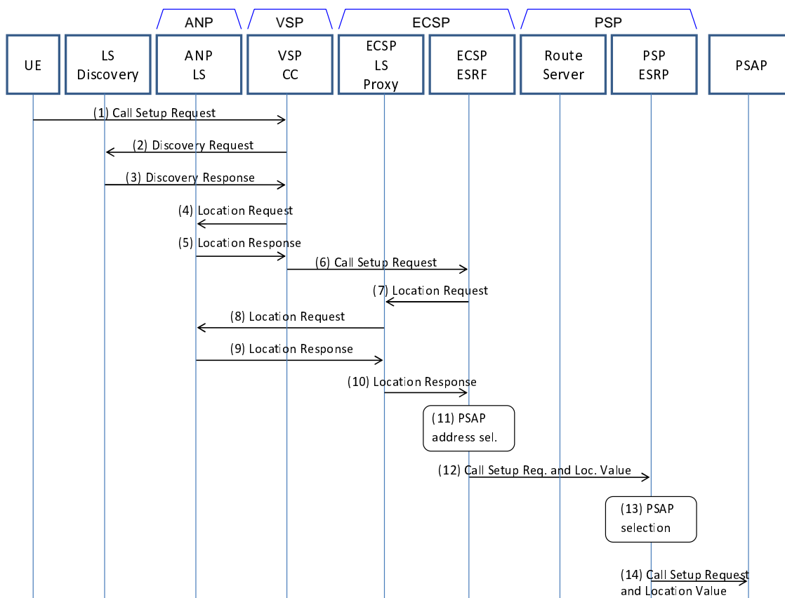
Figure 5.3: Call routing and location provisioning procedure when ANP provides location reference
