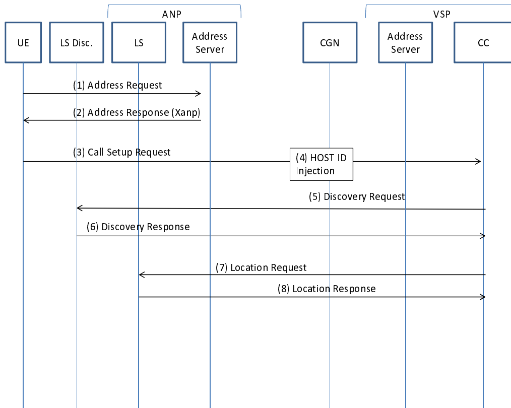
Figure A.5: Location retrieval with a CGN
