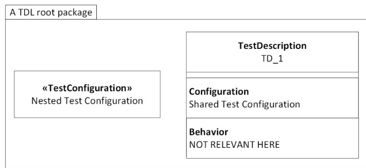
Figure 7: Concrete syntax representation of non-compositional references example
