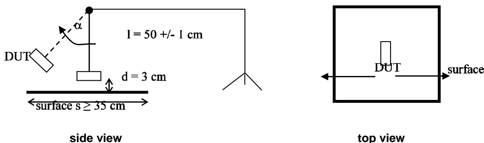
Figure 8: Positioning of handset under test
