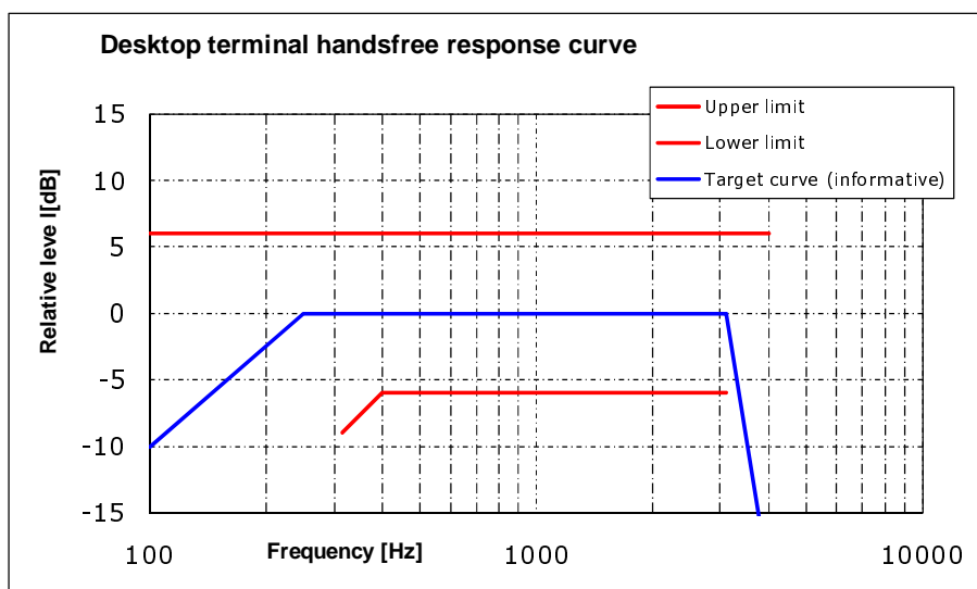
Figure 14: Receive frequency response dB mask for Desktop hands free terminals
