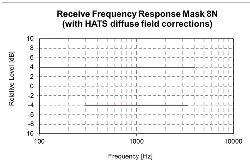
Figure 5: Receive frequency response mask for 8 N application force
