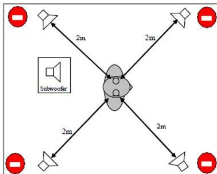
Figure 2: Loudspeaker arrangement in standard office rooms
