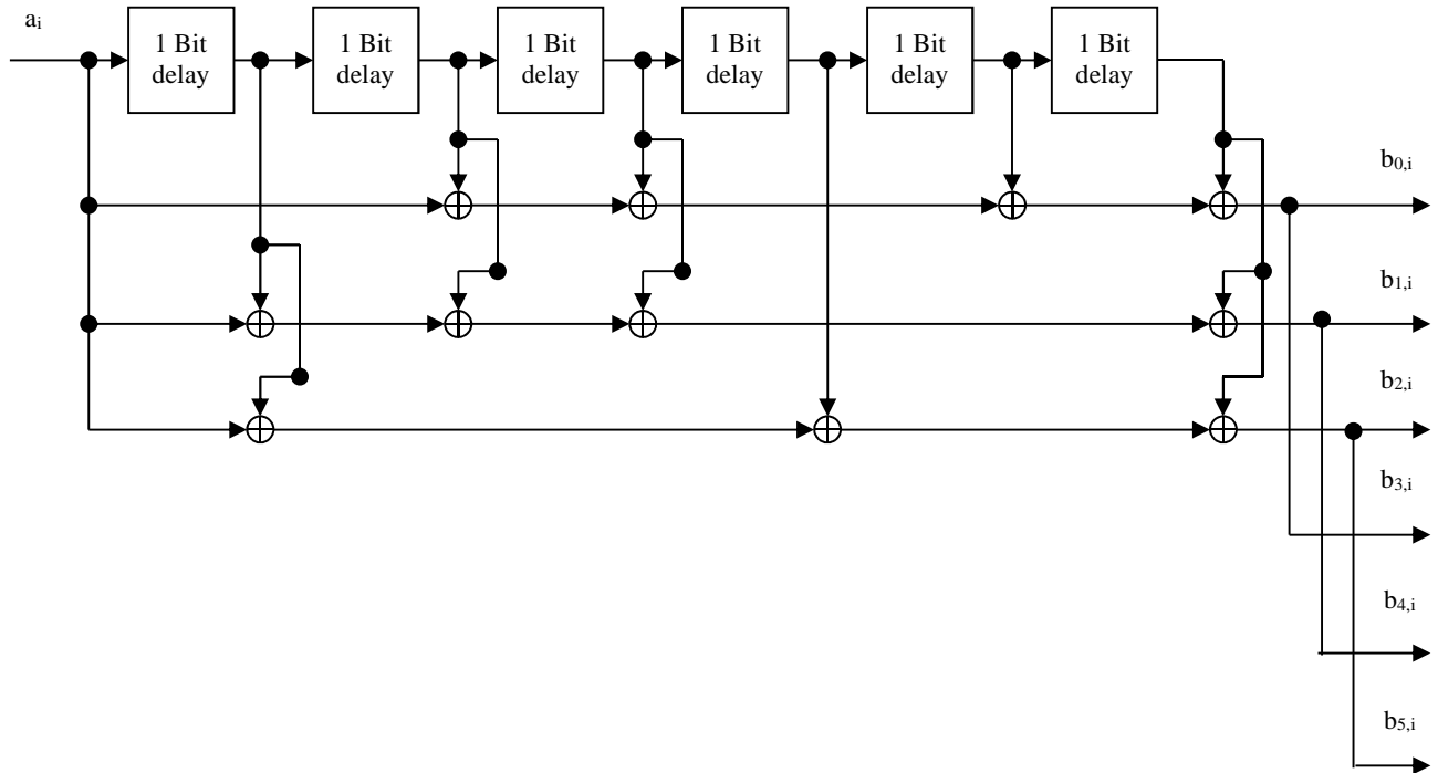
Figure 25: Convolutional encoder
