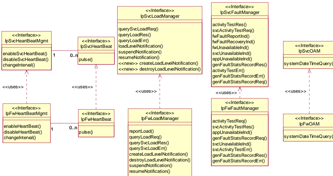
Figure 26: Integrity Management Package Overview
