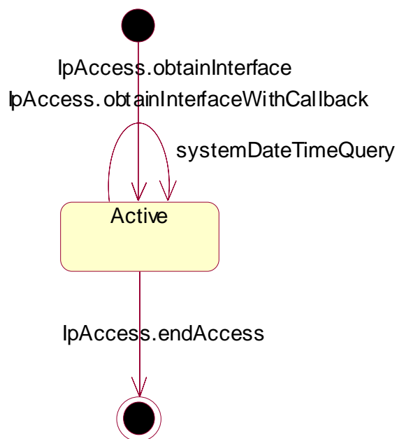
Figure 13: State Transition Diagram for IpOAM
