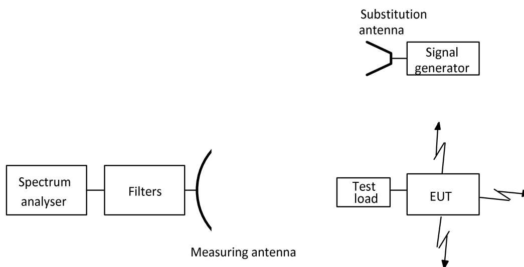
Figure 4: Test arrangement - spurious radiation measurements above 1 000 MHz for an EUT without antenna
