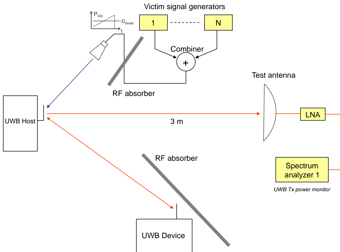
Figure 18: Example Setup for radiated DAA measurements
