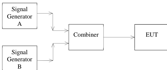
Figure 2: Blocking measurement arrangement
