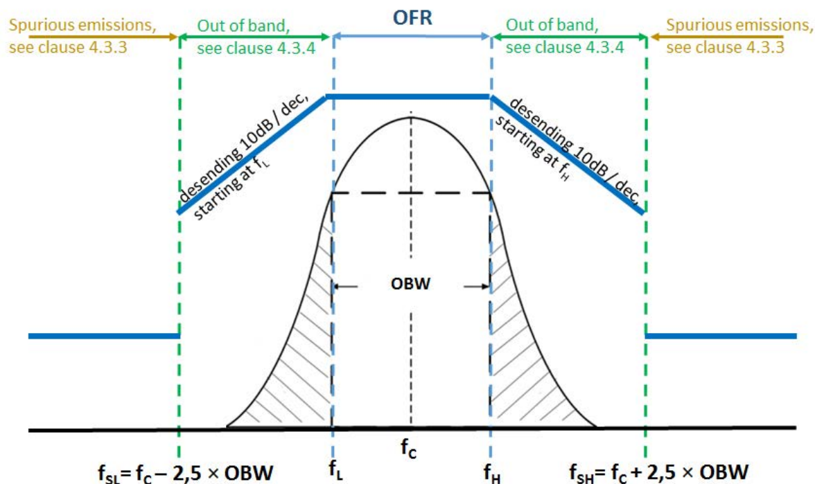
Figure 3: Out of band and spurious domain of a single frequency system
