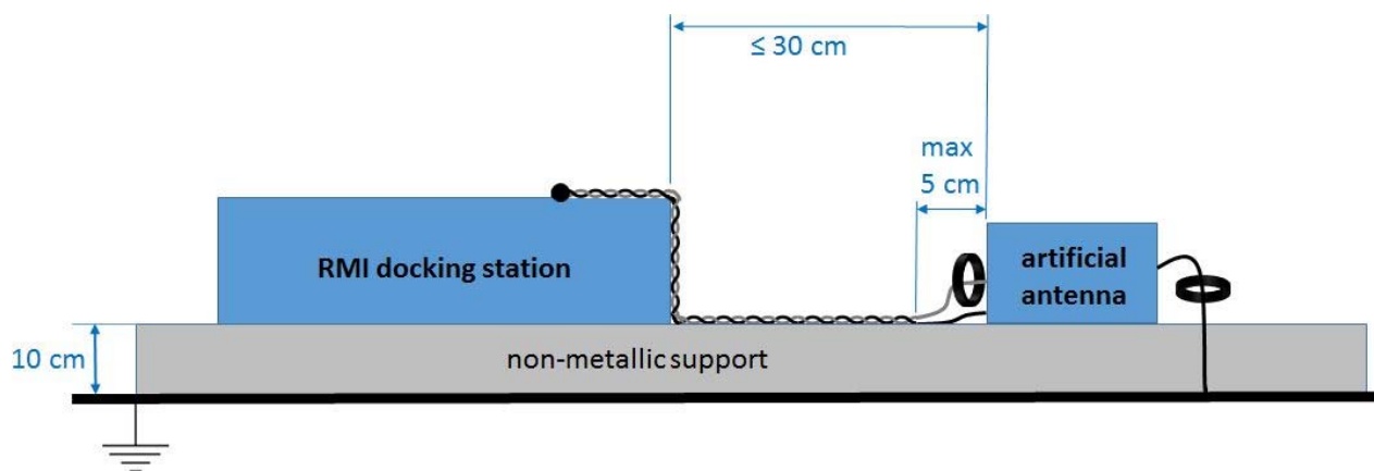
Figure C.3: Mechanical setup for artificial antenna
