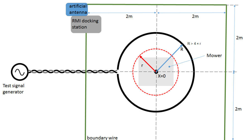
Figure 5: Schematic test set-up for the RX-blocking test 1
