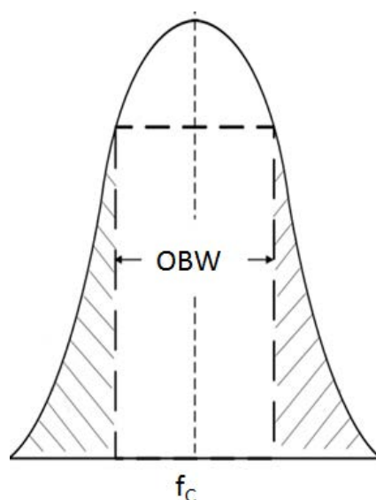
Figure 1: Occupied bandwidth (OBW)
