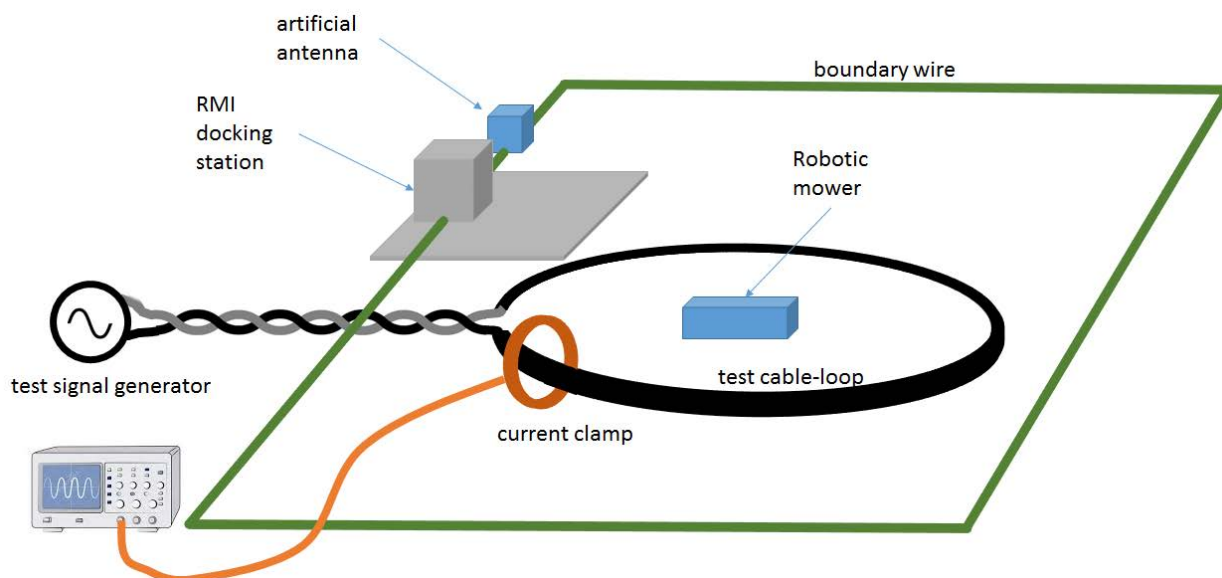
Figure 4: Schematic test set-up for the RX-blocking test 1
