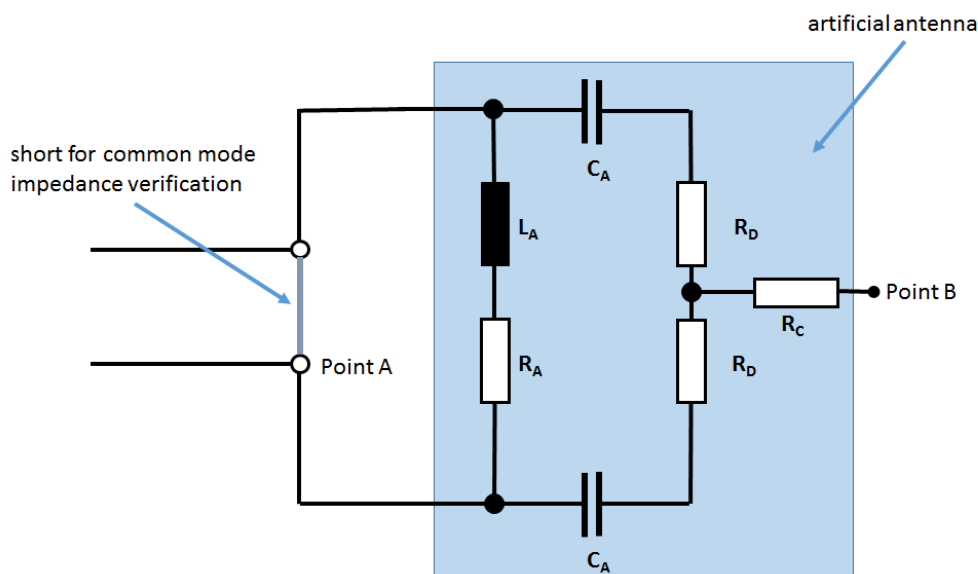
Figure C.2: Schematic for the verification of the artificial antenna common mode impedance
