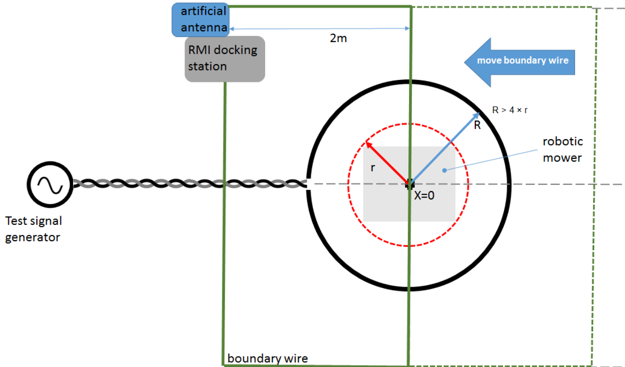
Figure 6: Schematic test set-up for the RX-blocking test 2
