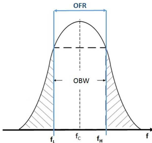
Figure 2: Operating Frequency Range (OFR)
