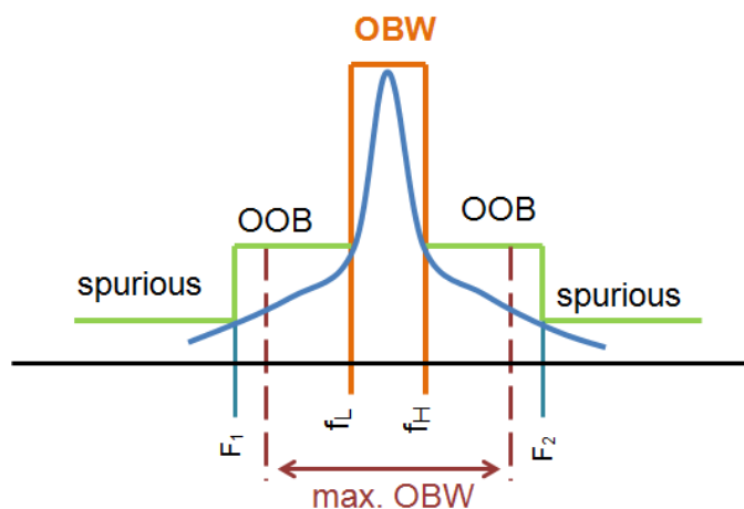
Figure 2: Overview OOB/spurious, depending on OBW
