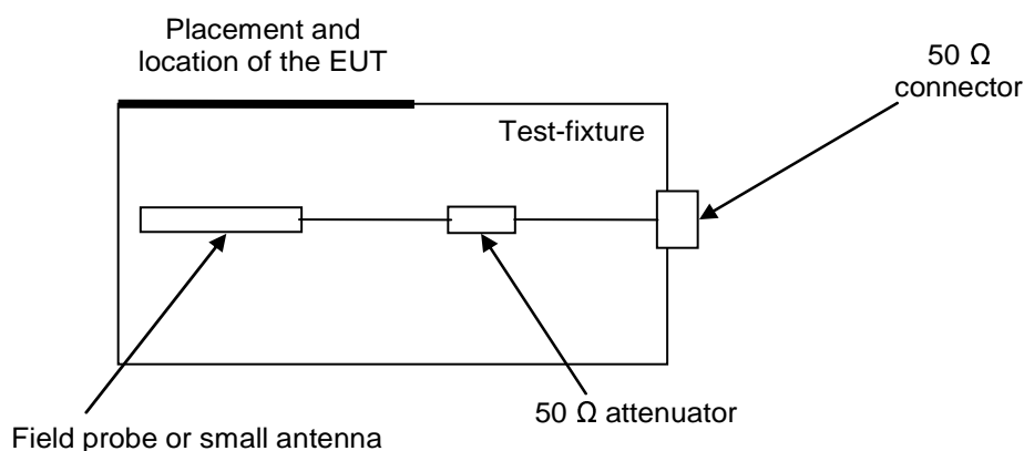
Figure A.4: Test fixture
