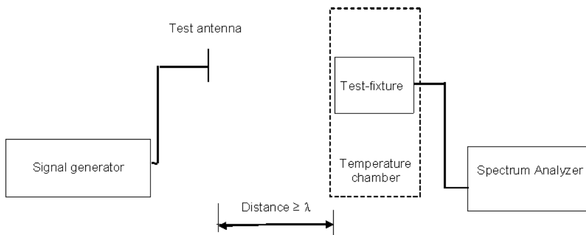
Figure A.5: Validation of test fixture without EUT
