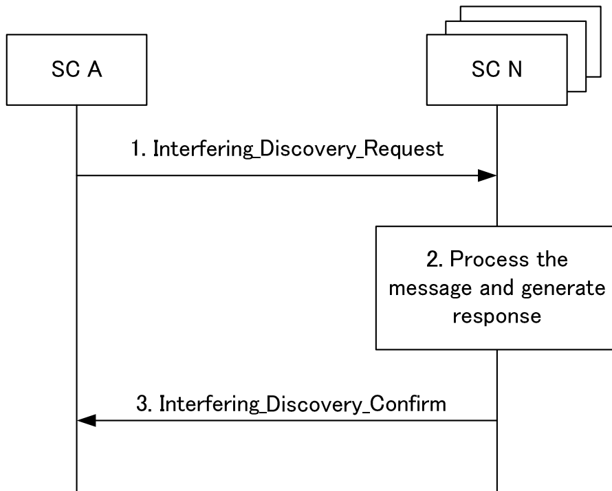
Figure 6.43: Interfering SC Discovery Procedure
