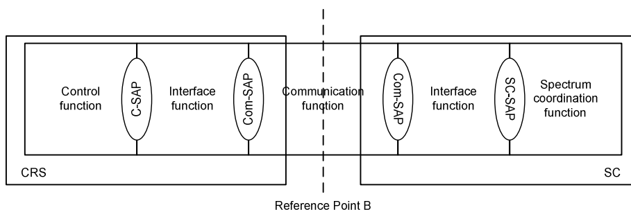
Figure 5.9: Reference point B
