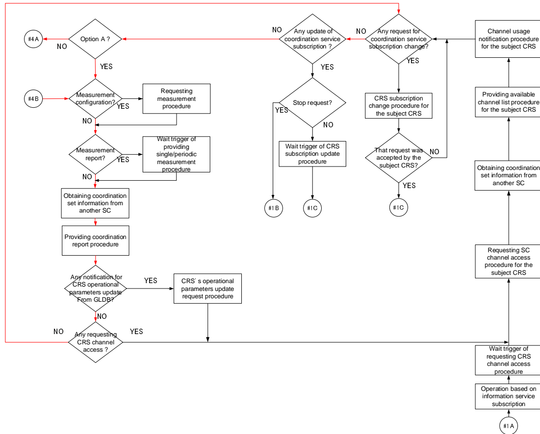
Figure 7.6: Information Service Operation
