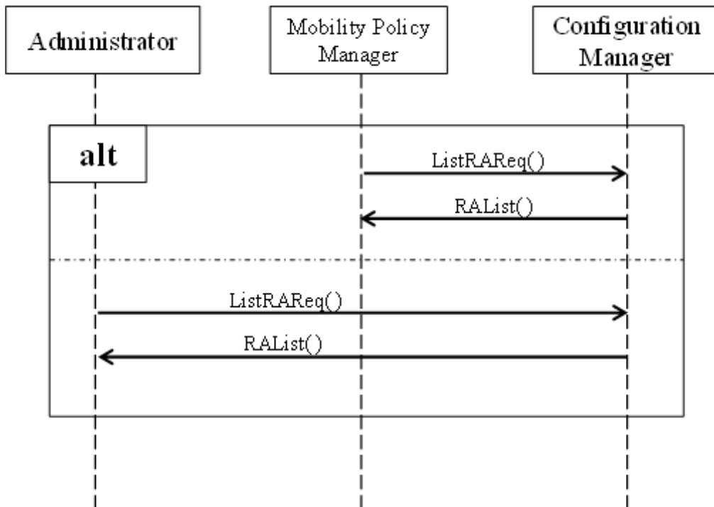
Figure 6.3: URA list checking
