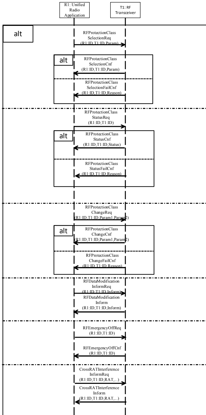
Figure 6.20: RVM protection services
