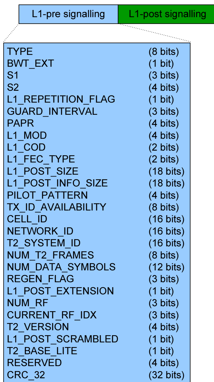
Figure 25: The signalling fields of L1-pre signalling
