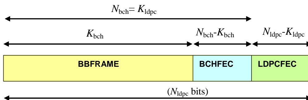
Figure 12: Format of data before bit interleaving ( N_{\text{ldpc}} = 64\ 800 bits for normal FECFRAME, N_{\text{ldpc}} = 16\ 200 bits for short FECFRAME)
