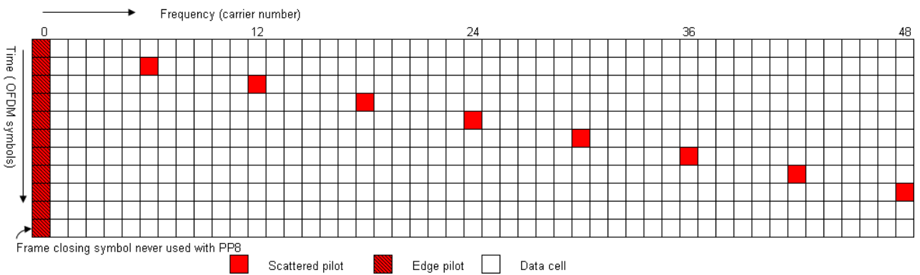
Figure K.8: Scattered pilot pattern PP8 (SISO)
