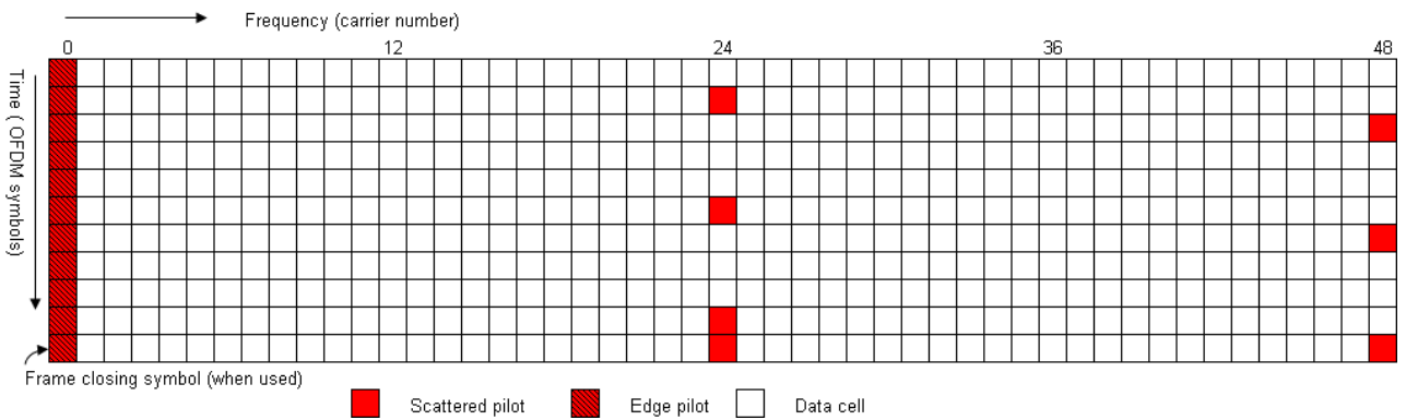
Figure K.7: Scattered pilot pattern PP7 (SISO)
