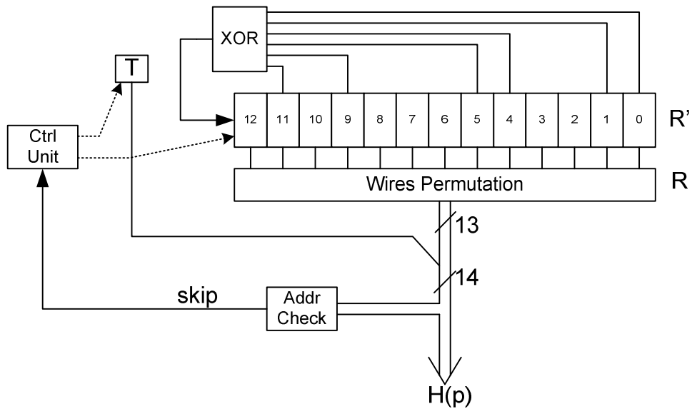
Figure 46(e): Frequency interleaver address generation scheme for the 16k mode
