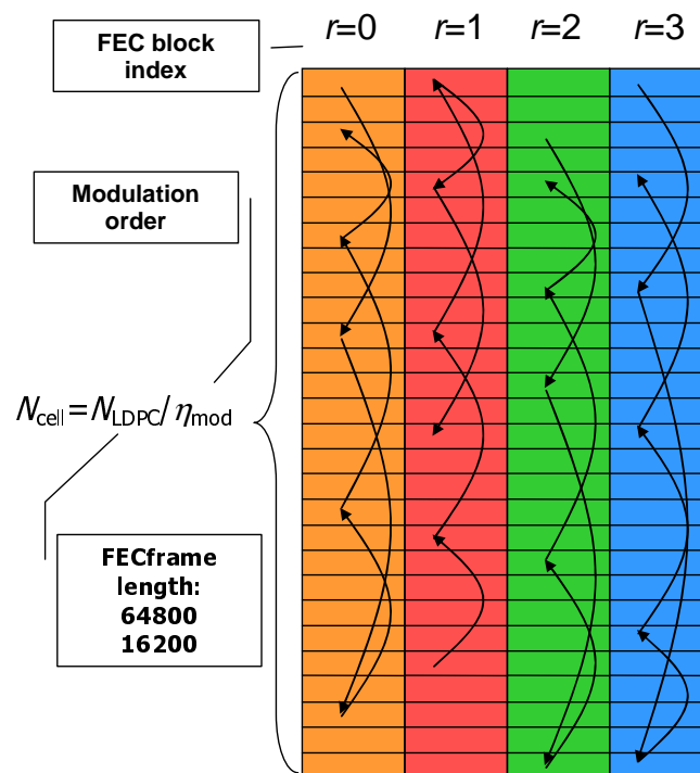
Figure 17: Cell Interleaving scheme
