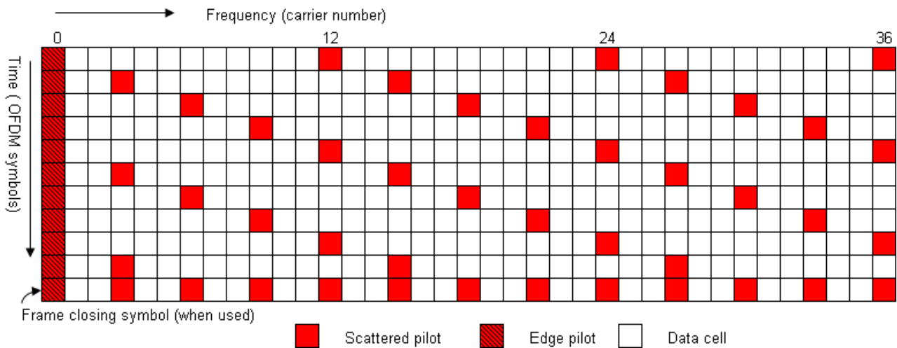
Figure K.1: Scattered pilot pattern PP1 (SISO)
