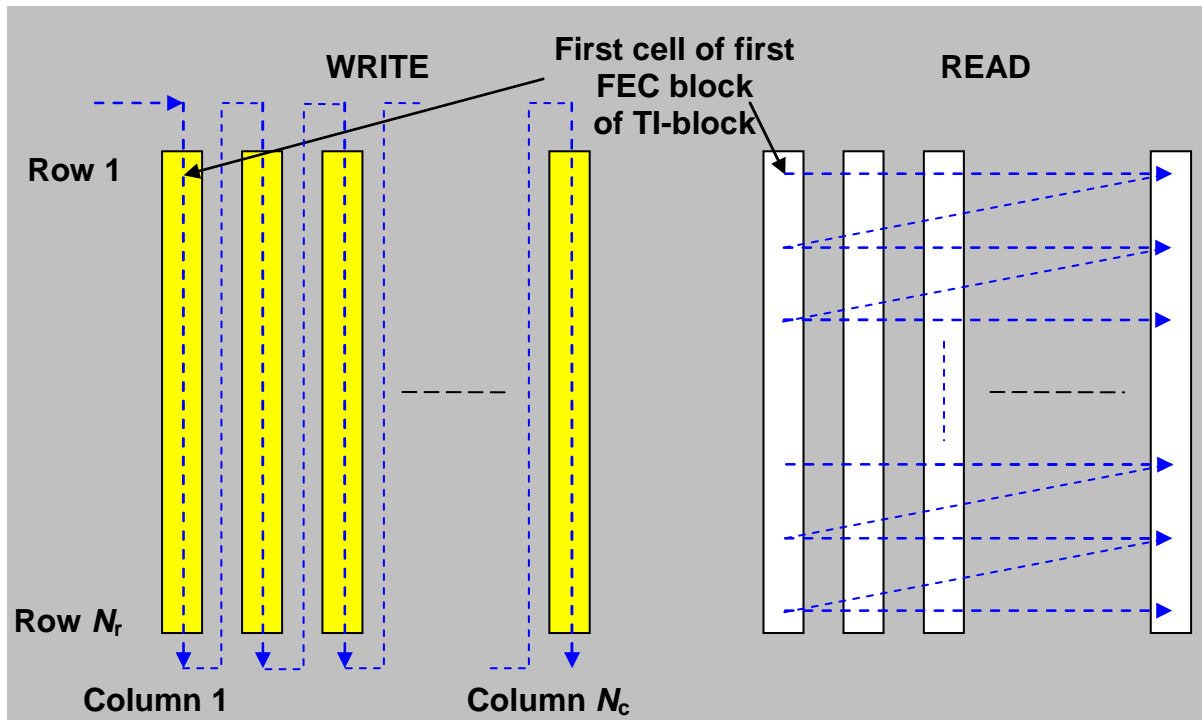
Figure 20: Time interleaver
