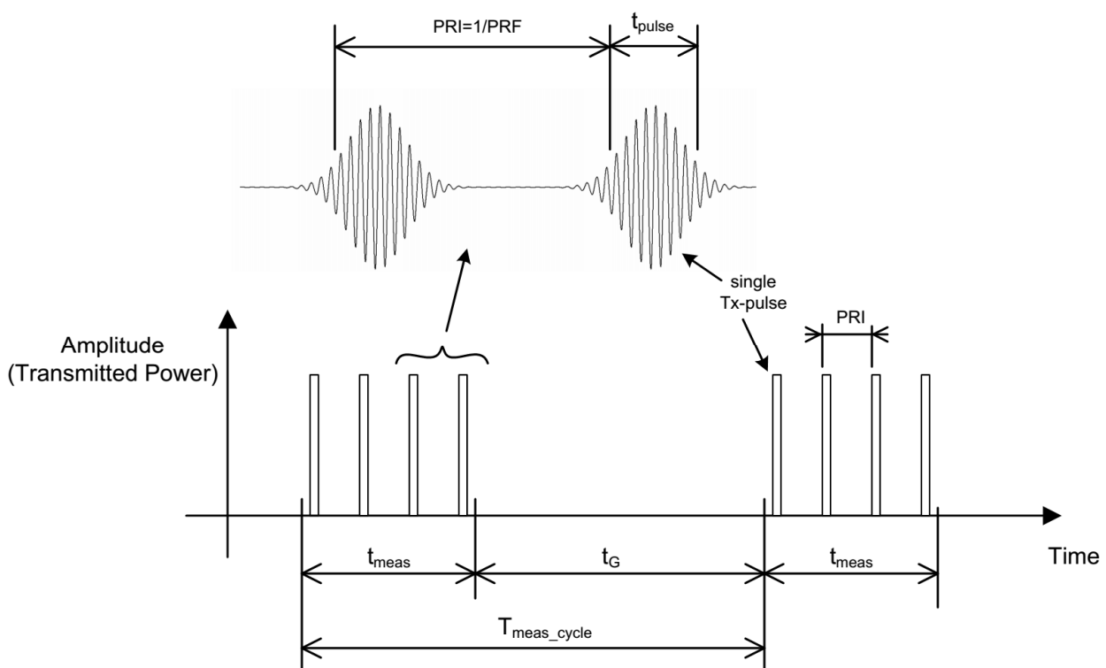
Figure H.1: Typical pulse modulation scheme
