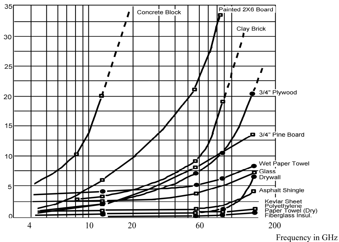
Figure I.3: Material Absorption at High Frequency in the frequency range from 3 GHz to 200 GHz in dB
