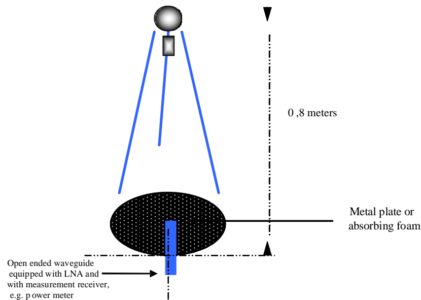
Figure 9: APC measurement setup
