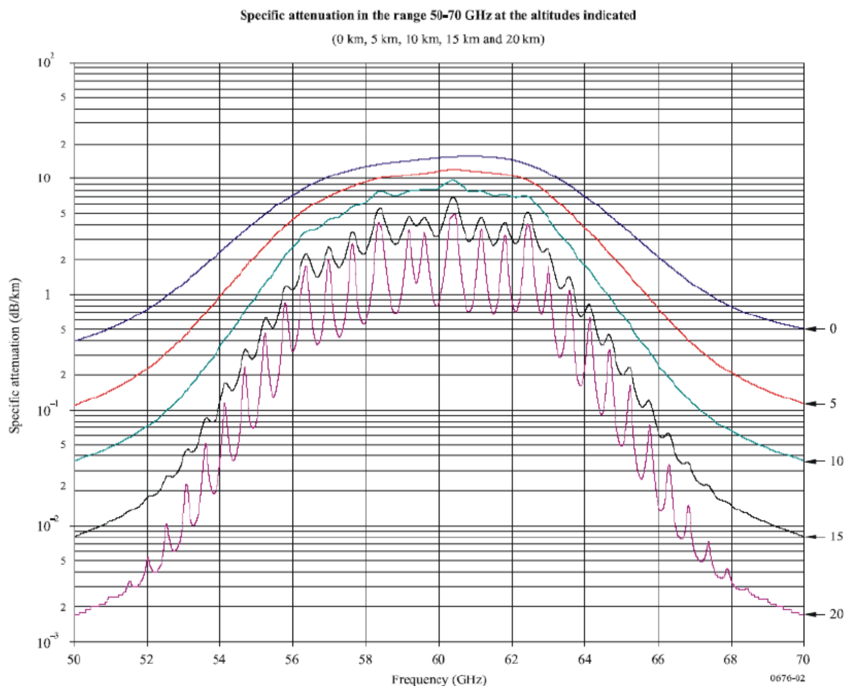
Figure I.2: Specific Atmospheric attenuation in the band 50 GHz to 70 GHz for different altitudes (0 km, 5 km, 10 km, 15 km and 20 km) [i.7]
