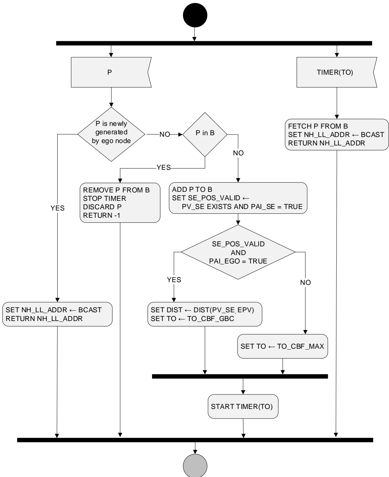
Figure F.1: Area contention-based forwarding algorithm
