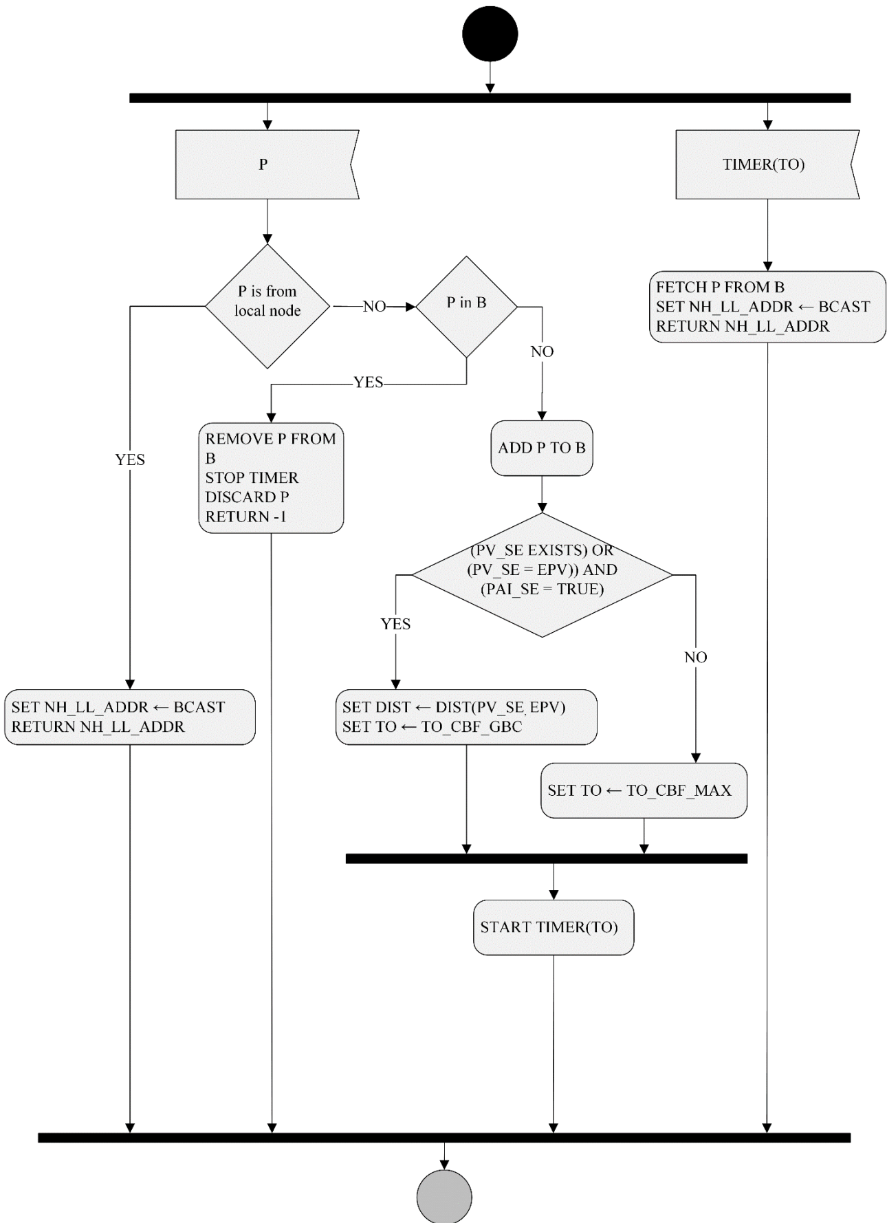
Figure F.1: Area contention-based forwarding algorithm
