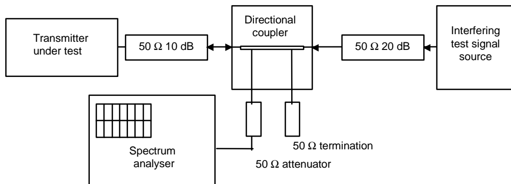
Figure 3: Measurement arrangement
