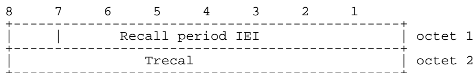
Figure 10.5/GSM 04.xx Recall period information element
