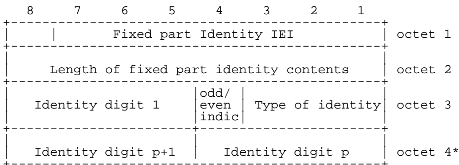
Figure 10.5/GSM 04.xx Fixed part Identity information element
