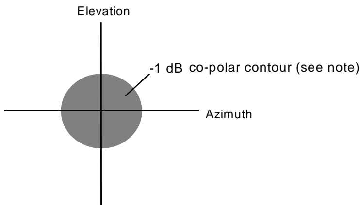
Figure 5: Category 2 mask for XPD measurements around the main beam axis
