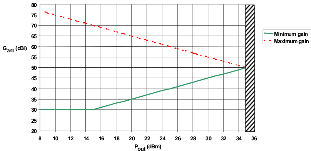
Figure UB.1: Graphical relationship among EIRP limitation, antenna gain and output power
