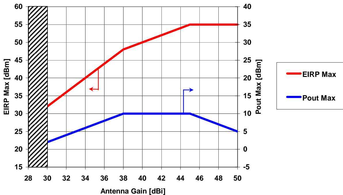
Figure UBa.1: Graphical relationship among EIRP limitation, antenna gain and output power
