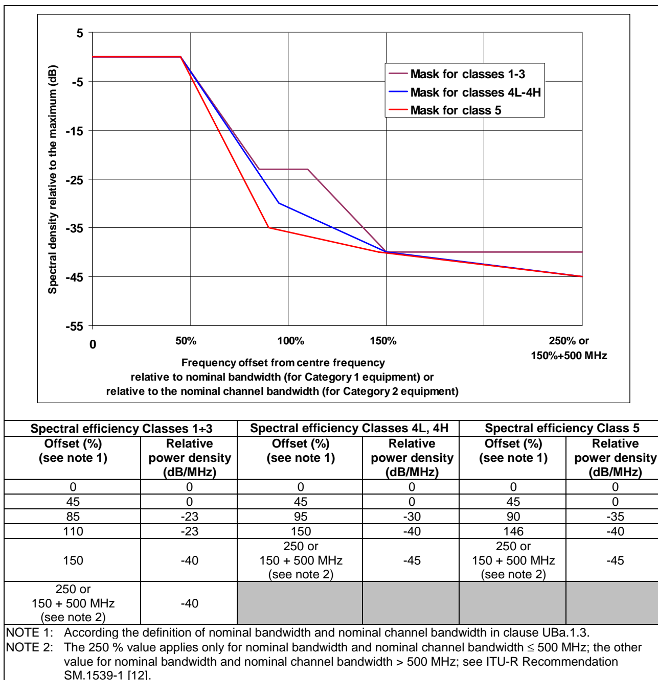
Figure UBa.3: TX EIRP spectral density mask
