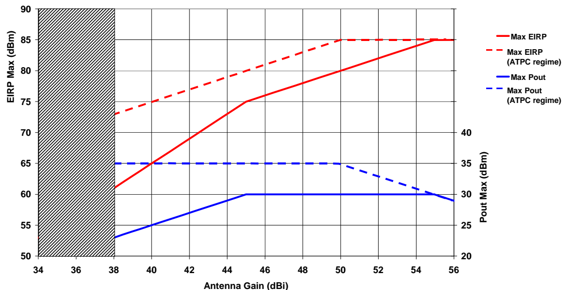
Figure UC.1: Graphical relationship among EIRP limitation, antenna gain and output power
