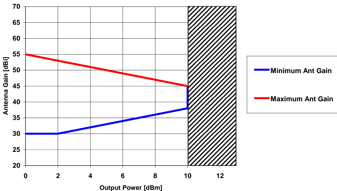
Figure UBa.2: Graphical relationship between actual output power and possible range of antenna gain for matching the EIRP limits (applicable to equipment with external antenna connector)
