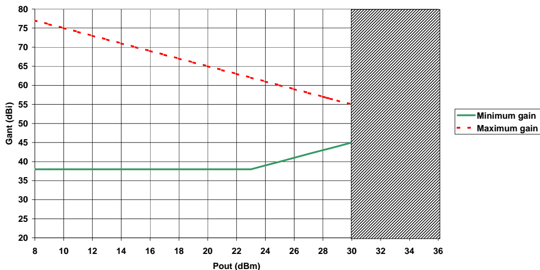
Figure UC.1: Graphical relationship among EIRP limitation, antenna gain and output power
