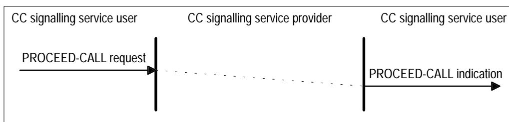
Figure 11: PROCEED-CALL service
