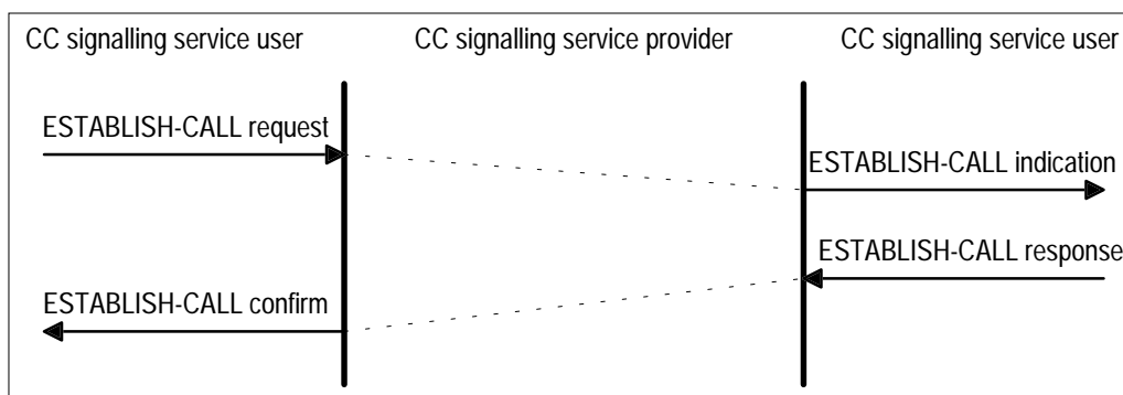
Figure 7: ESTABLISH-CALL service
