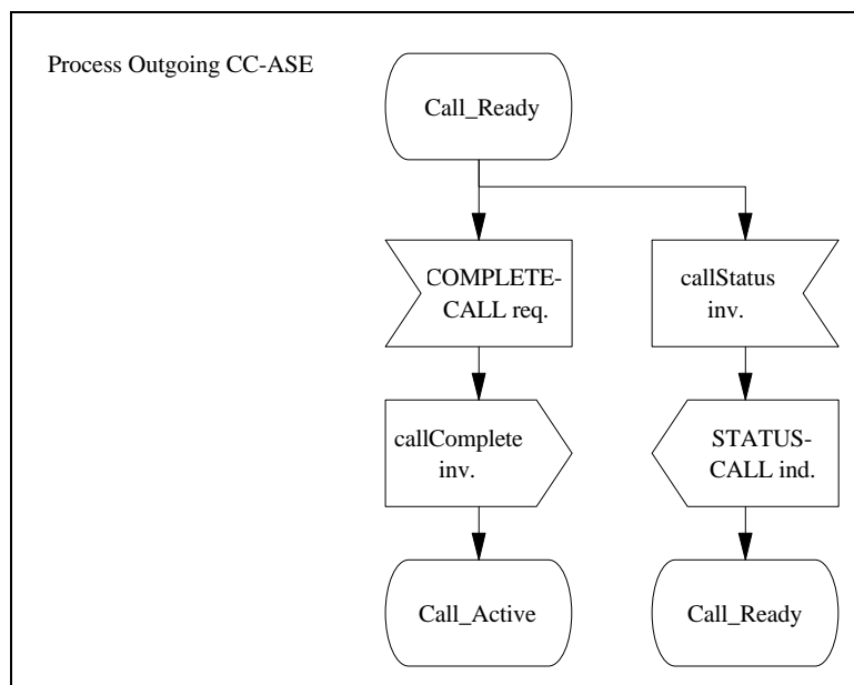
Figure 12.5: SDL for CC, outgoing call
