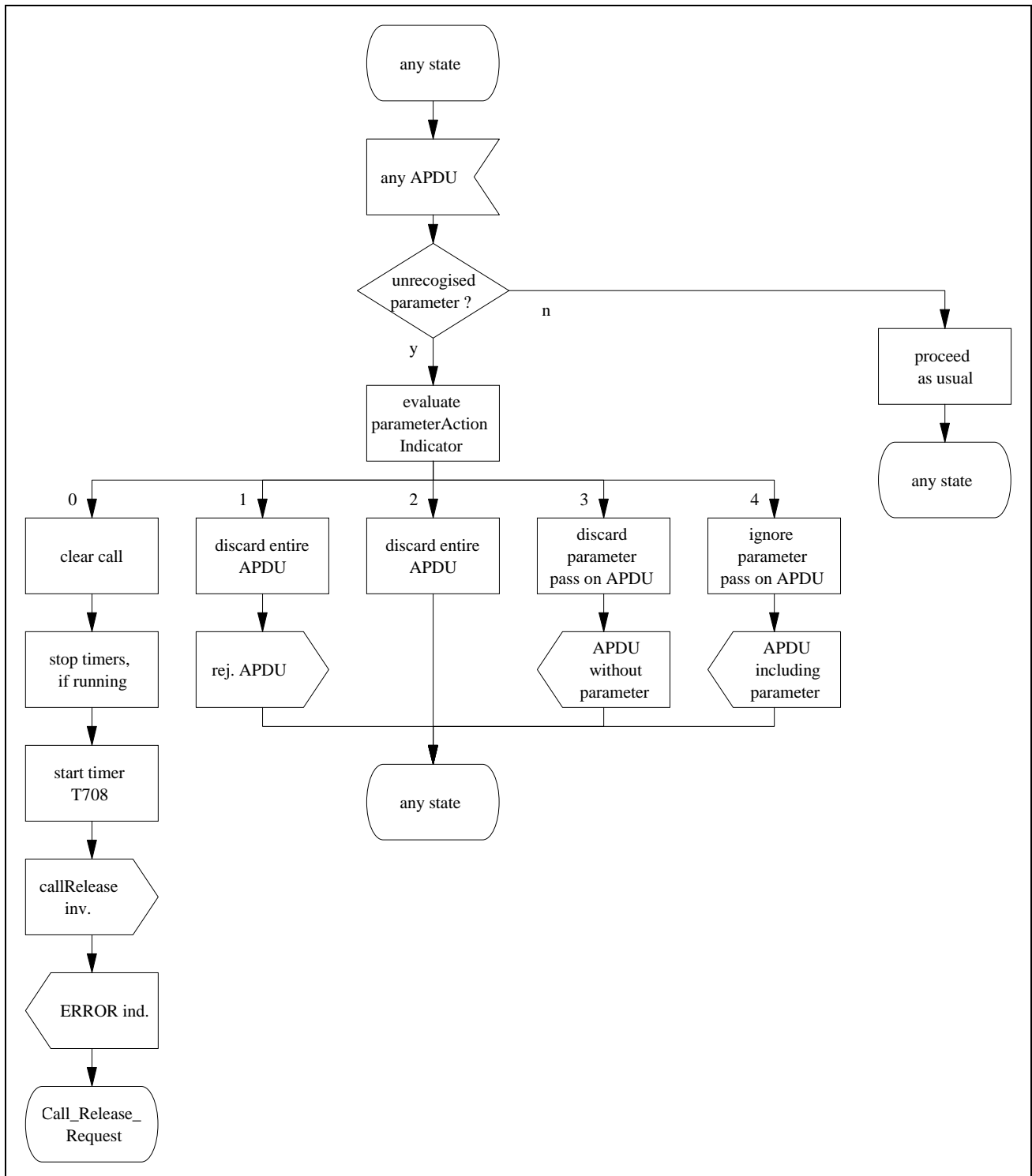
Figure 12.18: SDL for the handling of unrecognised parameters within CC operations
