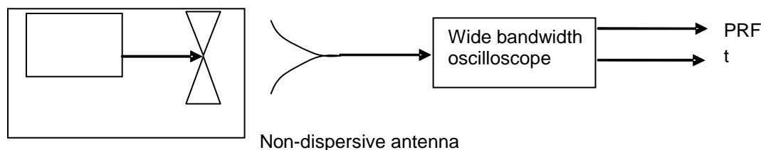
Figure F.1: Test setup 1
