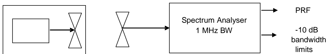
Figure F.2: Test setup 2
