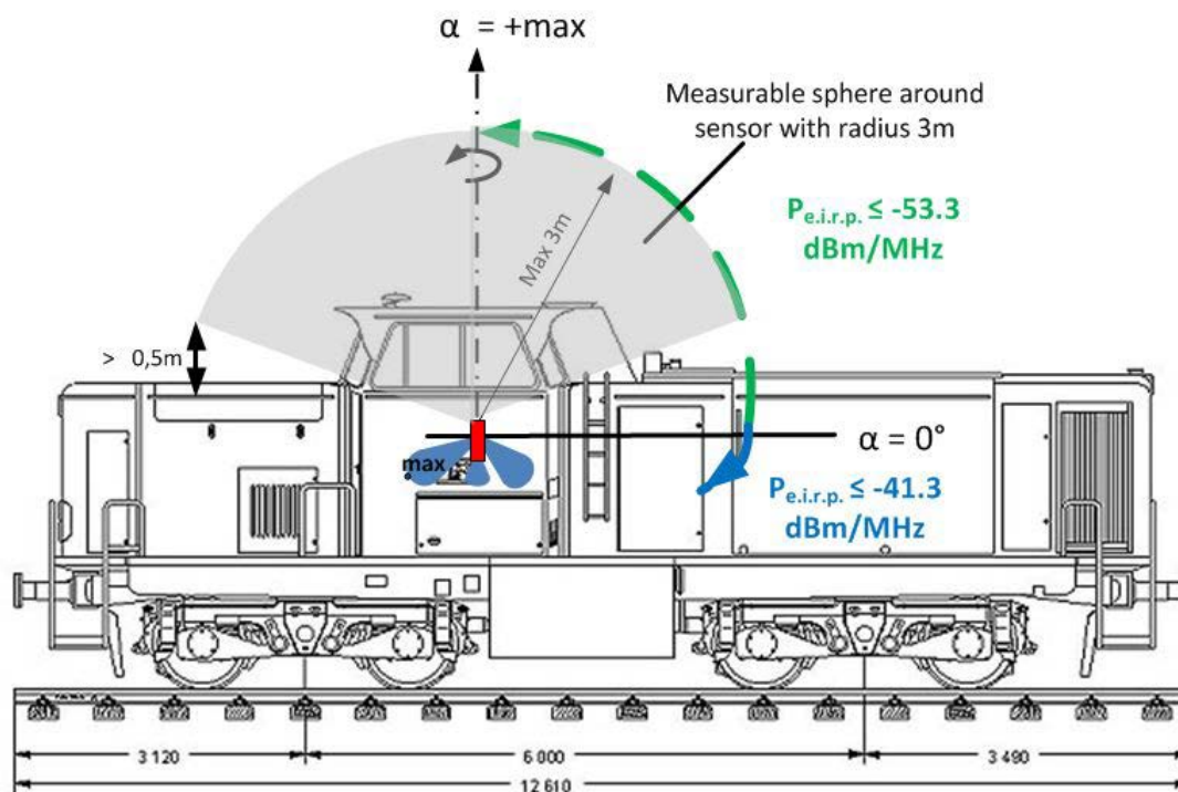
Figure 6: Example for an measurement spherical sector around an huge vehicle
