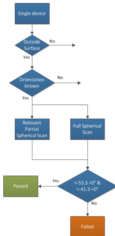
Figure C.1: Measurement Flow
