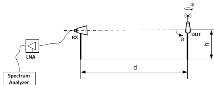
Figure 4: Spherical scan setup with rotation and tilt of the DUT
