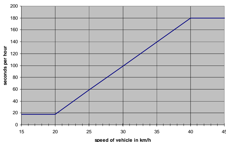
Figure 2: Long term duty cycle: Sum of transmitter on time with respect to speed of the vehicle [i.11]
