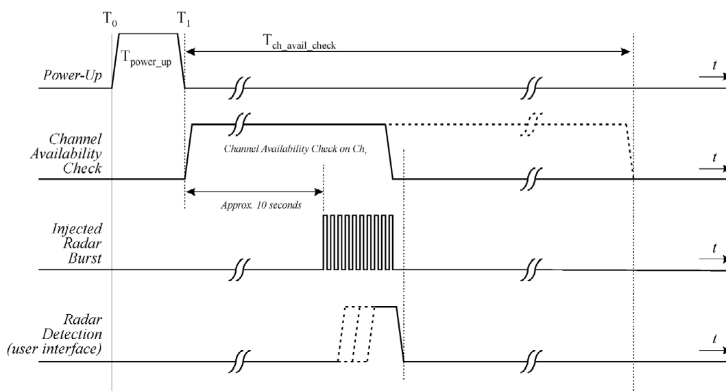
Figure 9: Example of timing for radar testing during the Channel Availability Check
