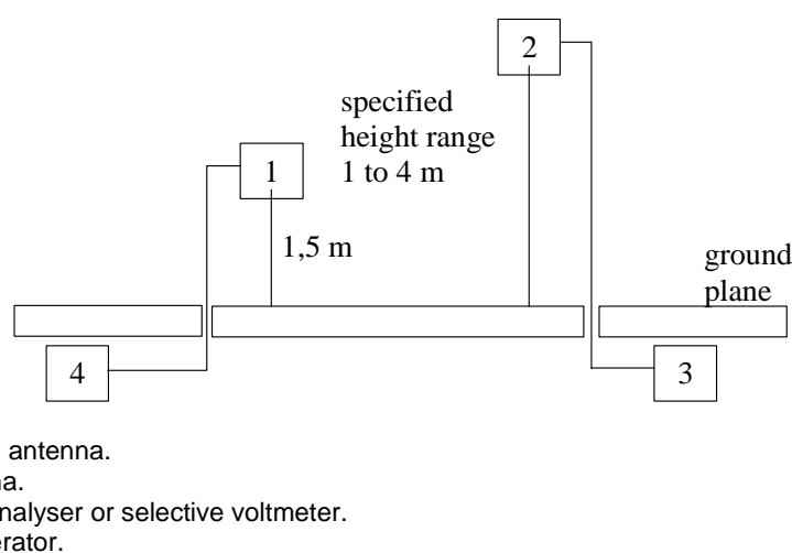
Figure C.2: Measurement arrangement 2
