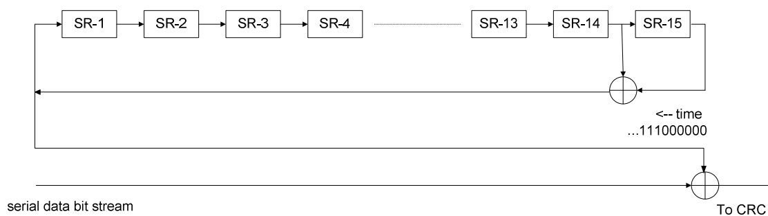
Figure 7-9: PRBS Randomizer
