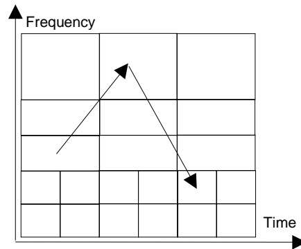
Figure 7-31: Dynamic MF-TDMA
