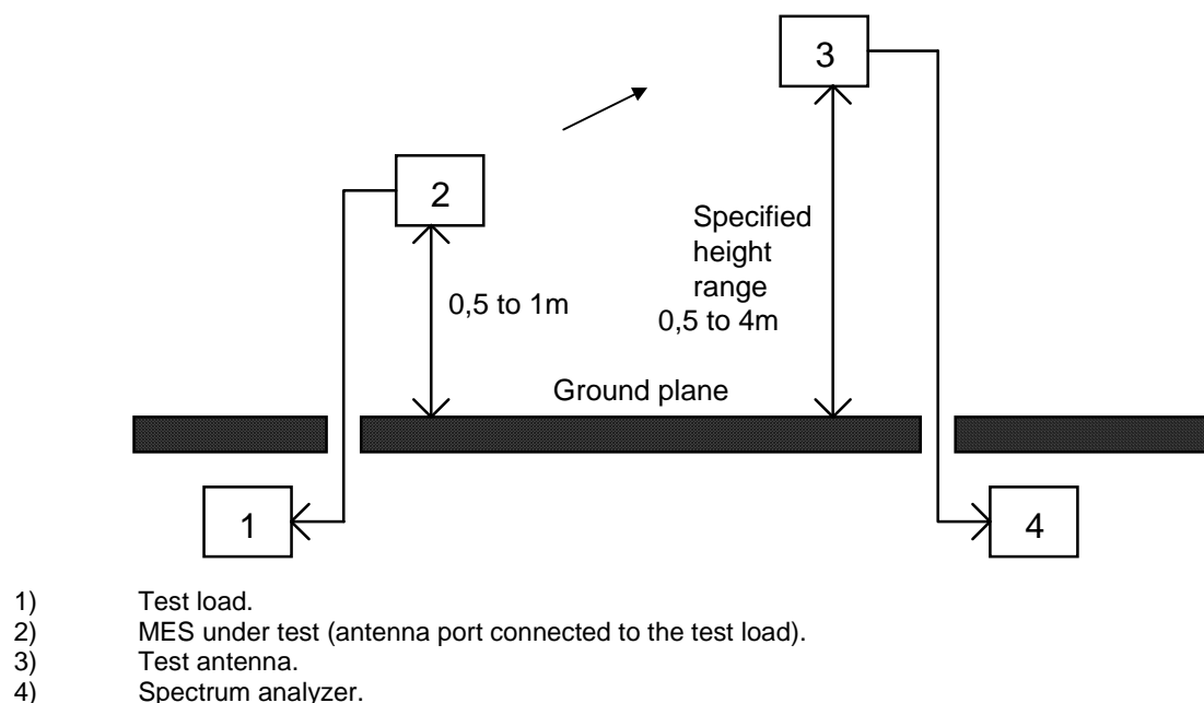
Figure 4: Measurement arrangement number 3
