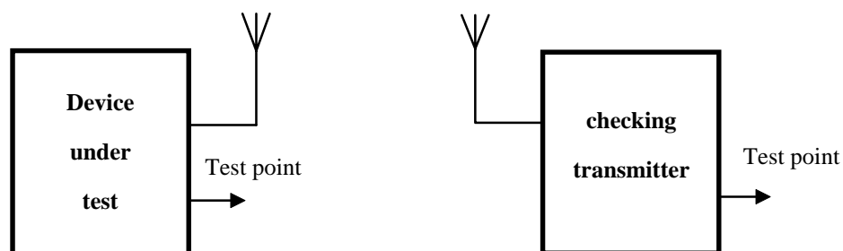
Figure 4: Measurement arrangement for a device's carrier sense delay measurement
