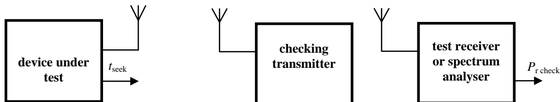
Figure 2: Measurement arrangement for evaluation of the anti blocking characteristic
