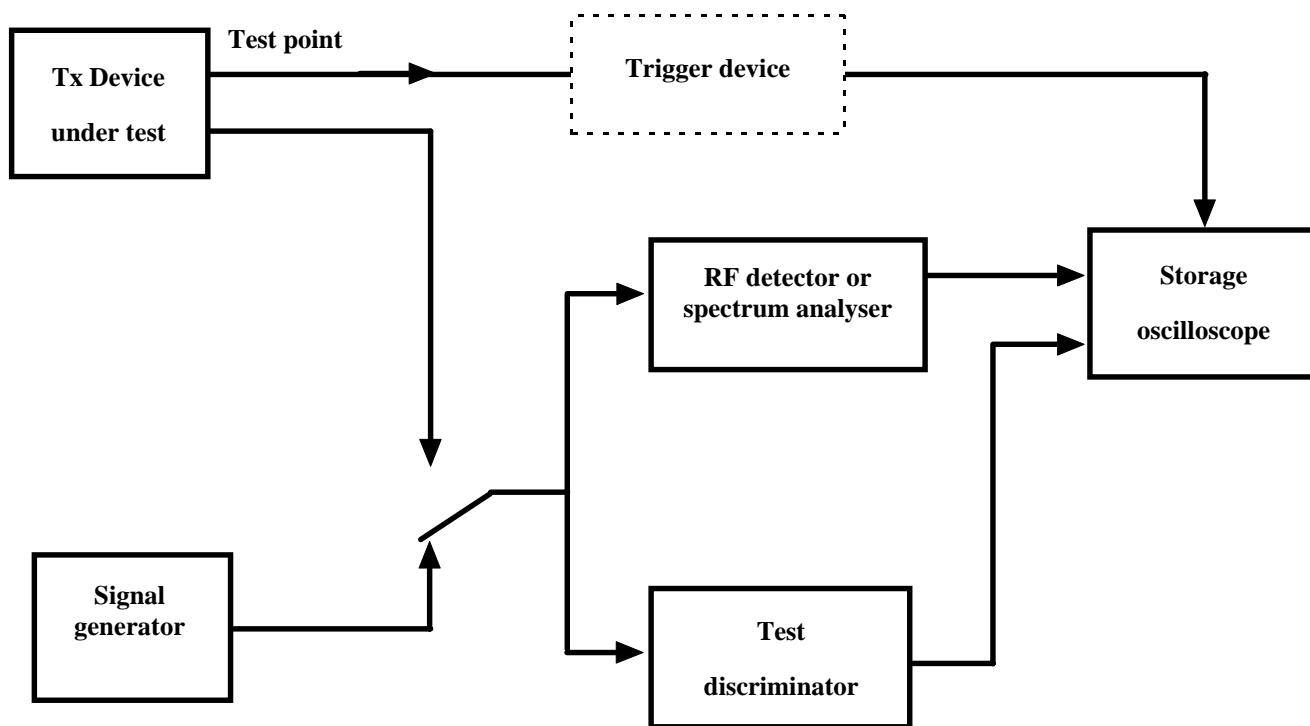
Figure 6: Measurement arrangement for the channel accessing carrier attack delay
