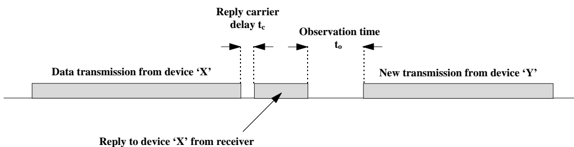
Figure 8: Channel access for a fixed rate of change of analogue level control
