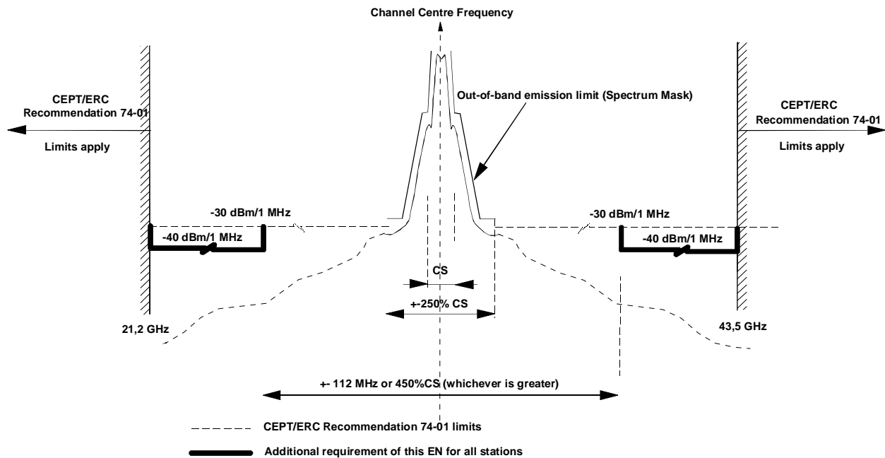
Figure 3: P-MP equipments for channel separation CS > 10 MHz
