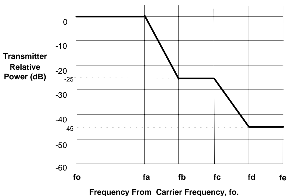
Figure 2: Limits of spectral power density as a function of channel spacing
