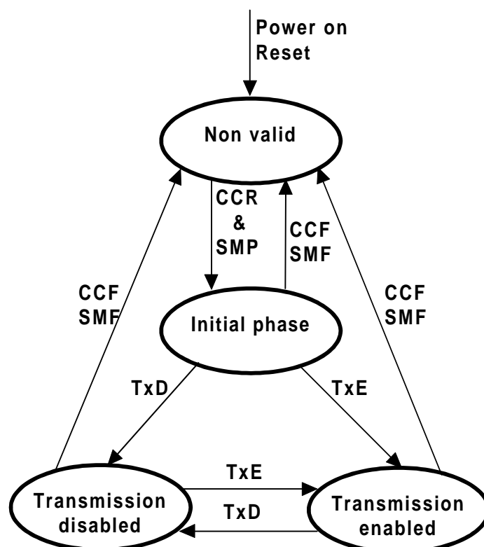
Figure 2: State transition diagram of the control and monitoring function of a SIT
