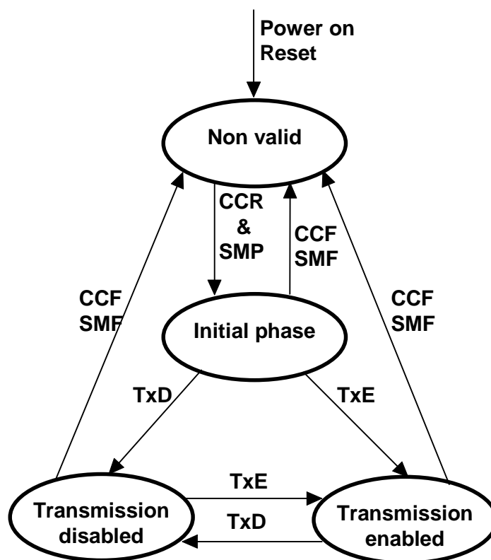
Figure 2: State transition diagram of the control and monitoring function of a SIT
