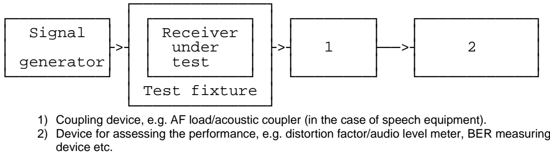
Figure A.5: Measuring arrangement for calibration
