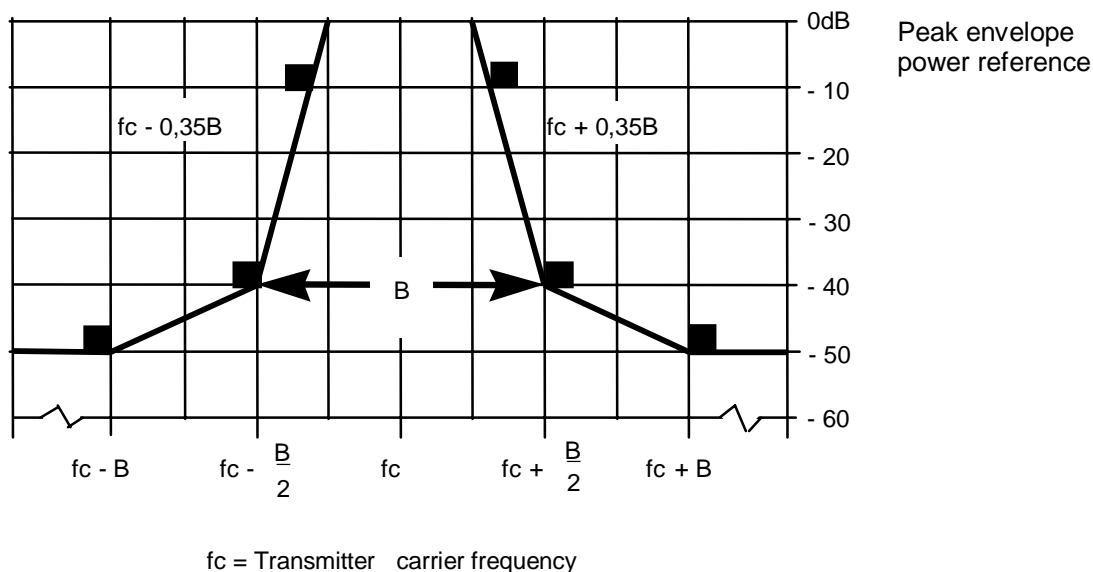
Figure 4: Scaleable Spectral mask for digital modulation with B = 600, 1 200kHz
