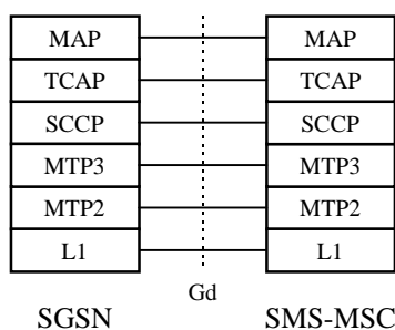
Figure 8: Signalling Plane SGSN - SMS-GMSC and SGSN - SMS-IWMSC
