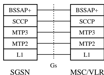
Figure 7: Signalling Plane SGSN - MSC/VLR
