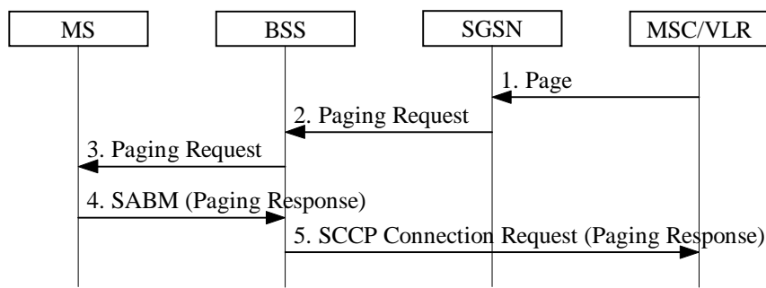
Figure 14: CS Paging Procedure
