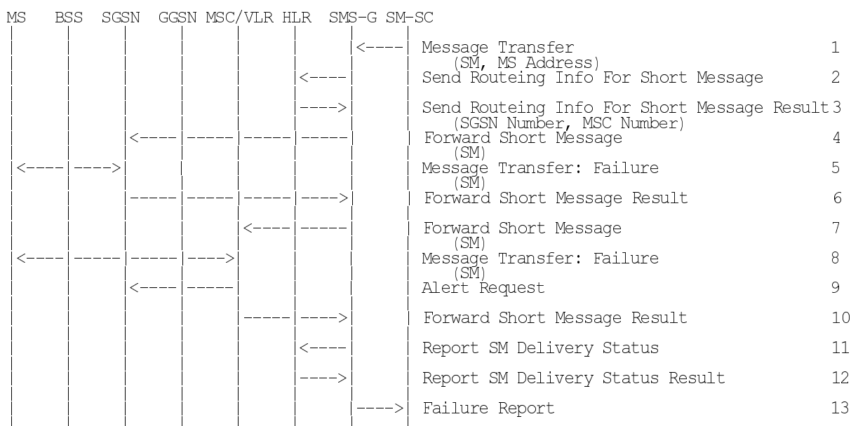
Figure 50: MT SMS Transfer, Unsuccessful
