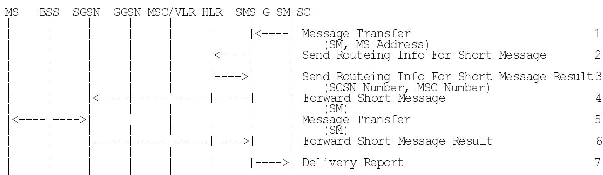
Figure 49: MT SMS Transfer, Successful
