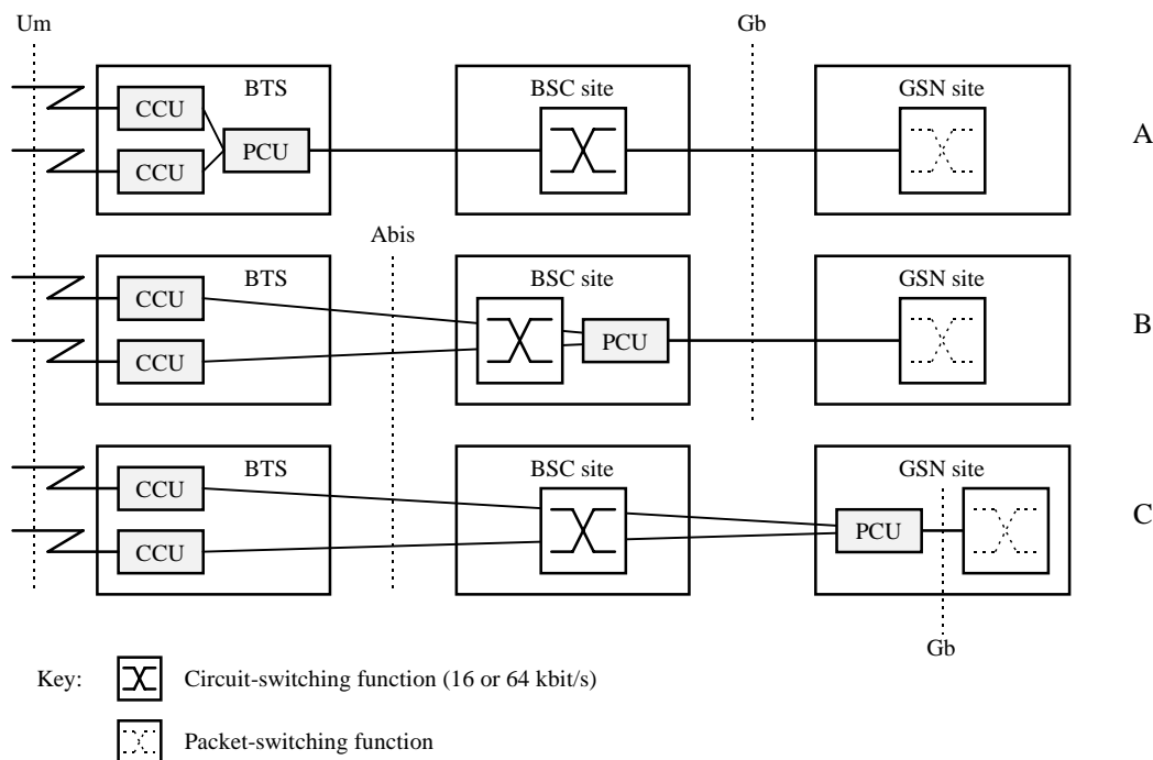
Figure 46: Remote Packet Control Unit (PCU) Positions
