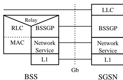
Figure 44: BSSGP Protocol Position
