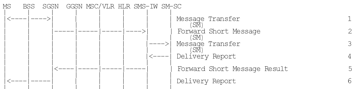
Figure 51: MO SMS Transfer, Successful
