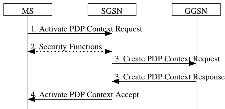
Figure 32: PDP Context Activation Procedure
