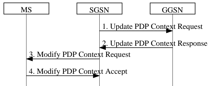
Figure 37: PDP Context Modification Procedure
