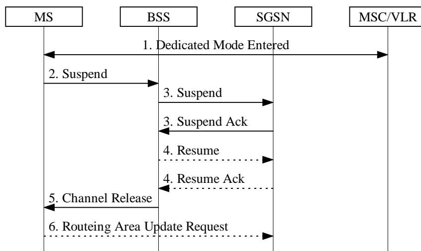
Figure 52: Suspend and Resume Procedure
