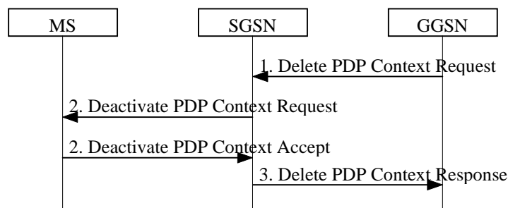
Figure 39: PDP Context Deactivation Initiated by GGSN Procedure
