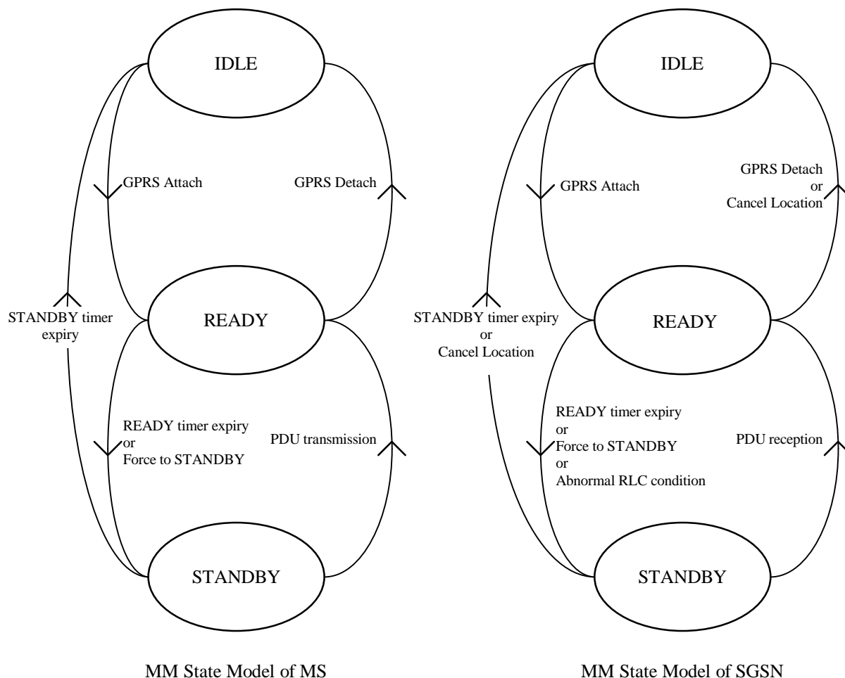
Figure 12: Functional Mobility Management State Model
