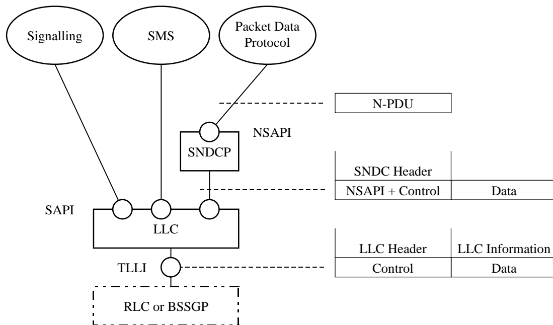
Figure 42: Multiplexing of Network Protocols
