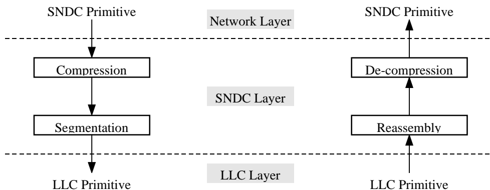
Figure 43: Sequential Invocation of SNDC Functionality
