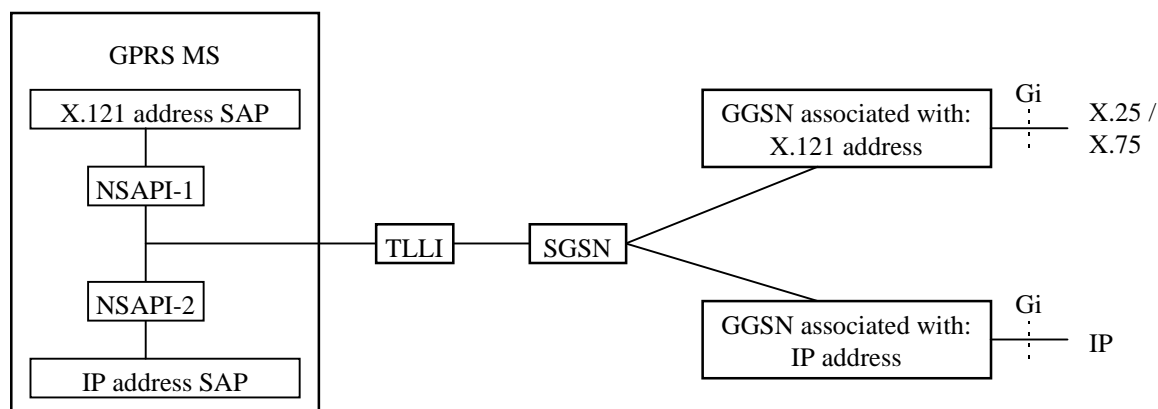
Figure 48: Use of NSAPI and TLLI
