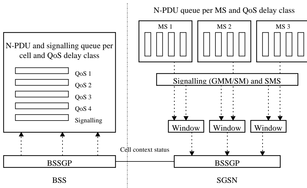
Figure 45: Flow Control of Downlink Traffic
