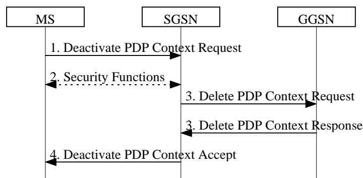
Figure 38: PDP Context Deactivation Initiated by MS Procedure
