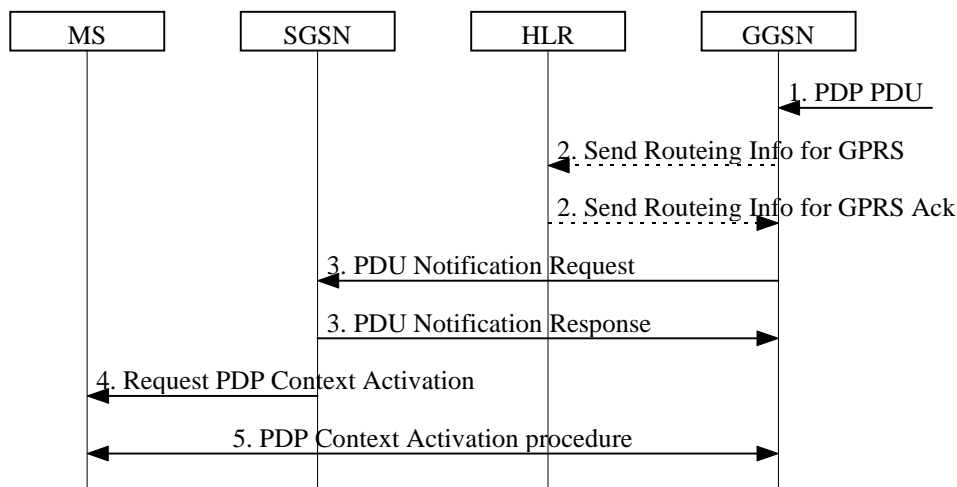
Figure 33: Successful Network-Requested PDP Context Activation Procedure
