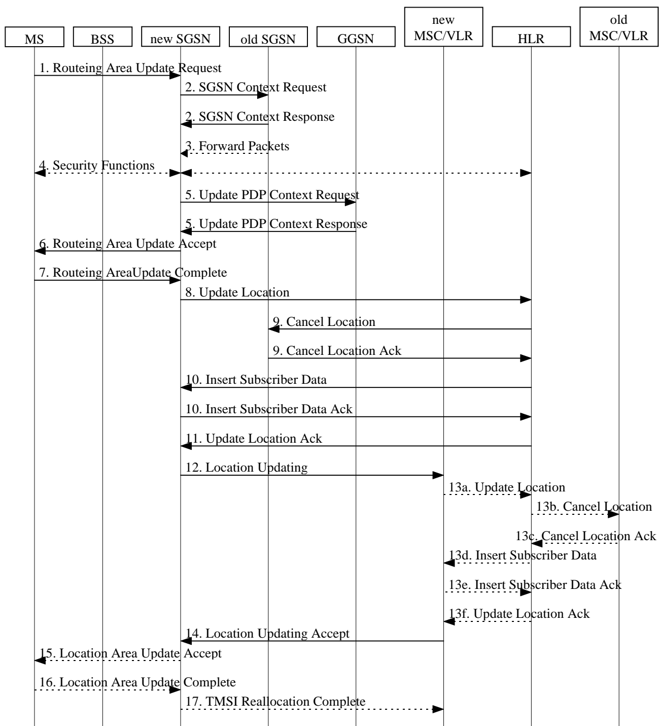
Figure C.1: Combined RA / LA Update in the Case of Inter SGSN RA Update Procedure, Optimised
