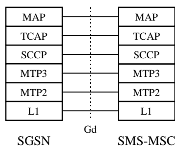
Figure 8: Signalling Plane SGSN - SMS-GMSC and SGSN - SMS-IWMSC
