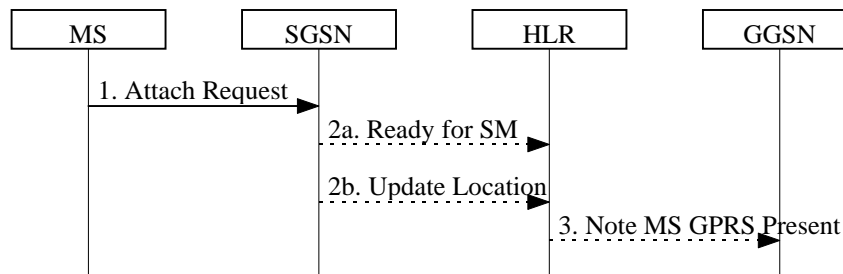
Figure 35: Mobile User Activity Procedure
