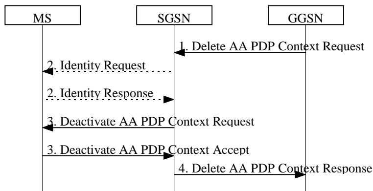
Figure 41: Anonymous Access PDP Context Deactivation Initiated by GGSN Procedure
