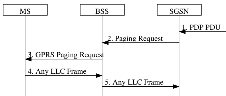
Figure 30: GPRS Paging Procedure
