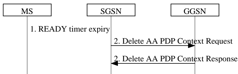
Figure 40: Anonymous Access PDP Context Deactivation Initiated by MS Procedure
