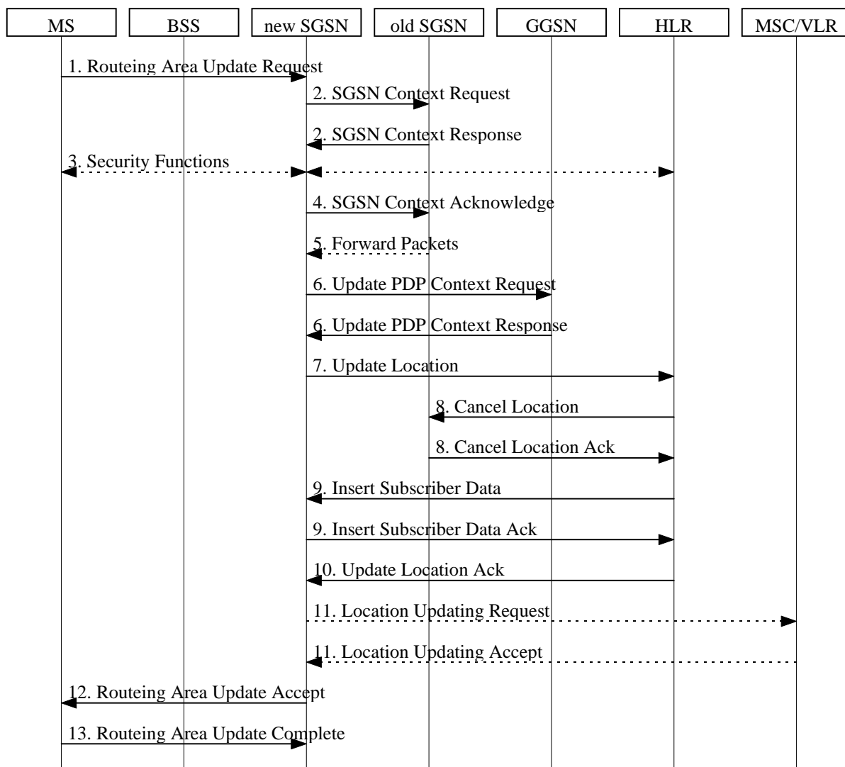
Figure 27: Inter SGSN Routing Area Update Procedure
